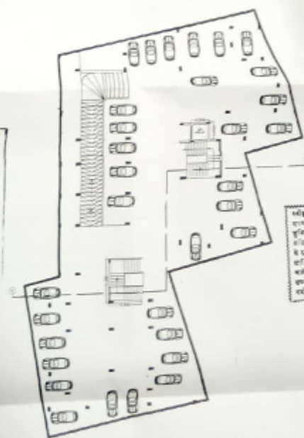
LOWER BASEMENT FLOOR PLAN
