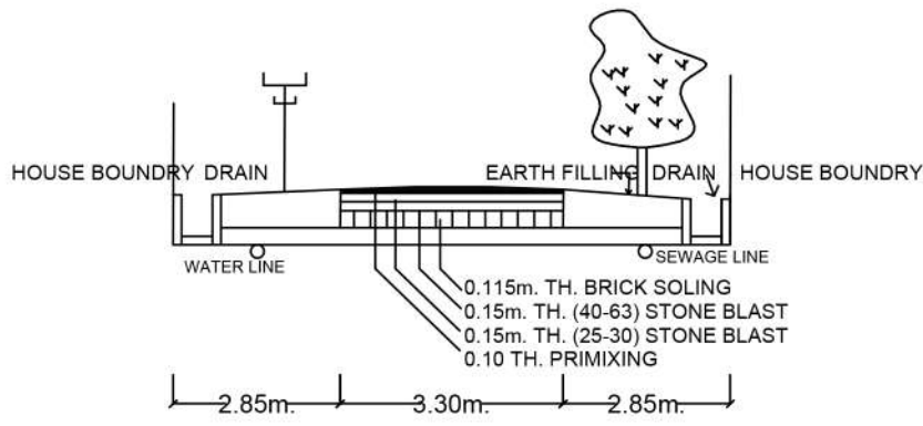
SECT. DETAILS OF 9.00M. WIDE ROAD
