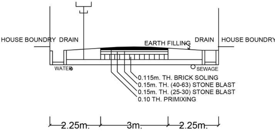
SECT. DETAILS OF 7.50M. WIDE ROAD
