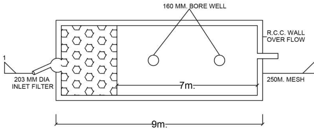
PLAN RAIN WATER HARVESTING
