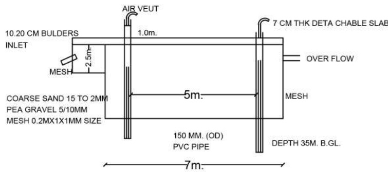
SECT. DETAIL AT 1-1
