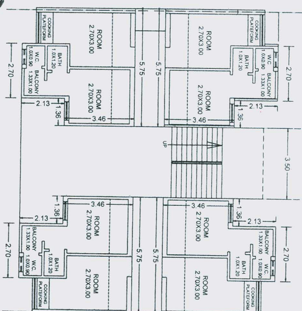
UNIT PLAN
