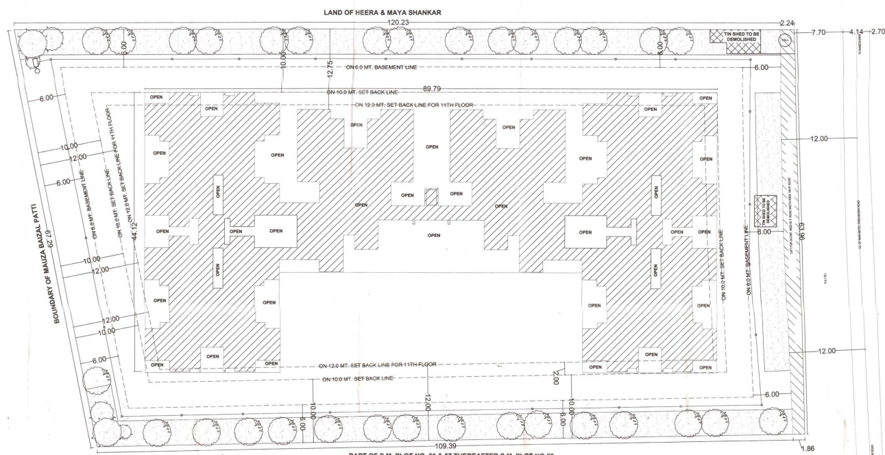
SITE PLAN & RAIN WATER HARVESTING PLAN
