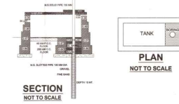
RAIN WATER HARVESTING PLAN NOT TO SCALE
