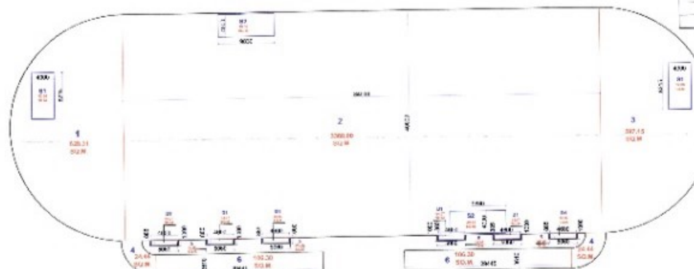
ENVELOPE PLAN OF LOWER GROUND FLOOR SCALE 1:150
