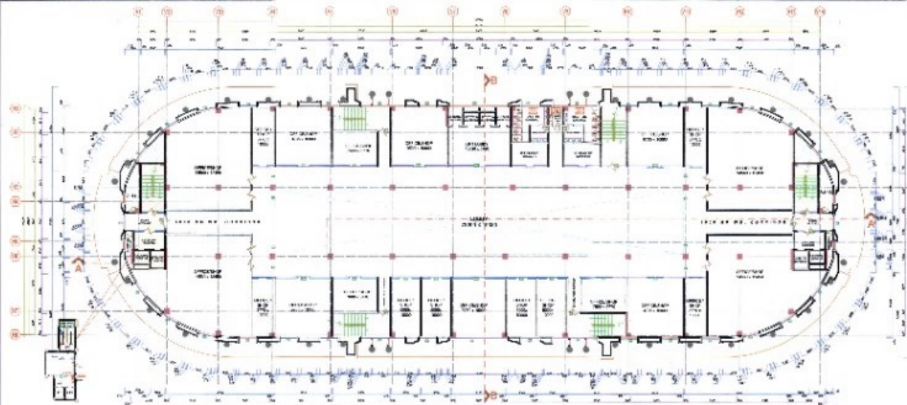
SIXTH FLOOR PLAN SCALE 1:150
