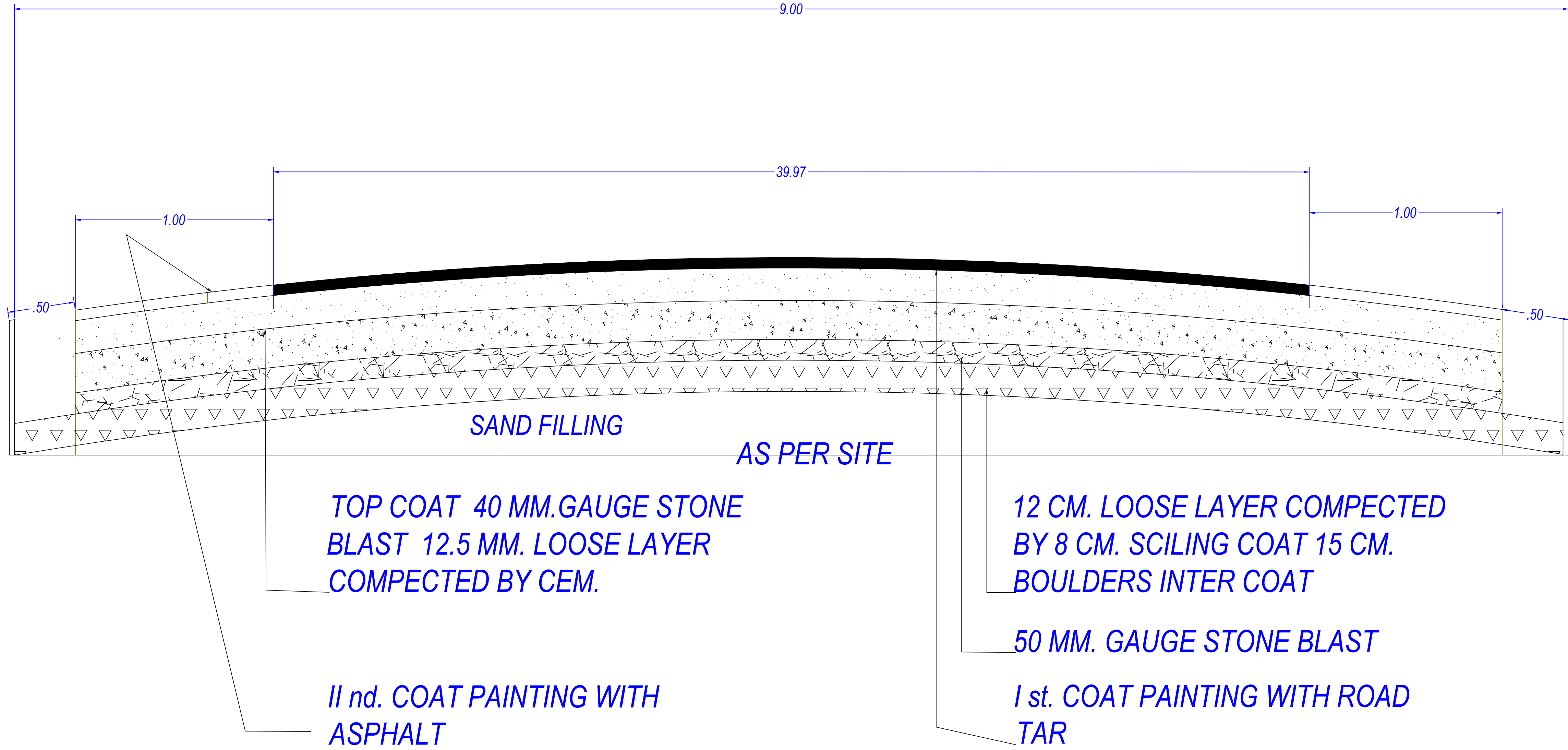
DETAIL OF ROAD SECTOIN SCALE:-N.T.S.
