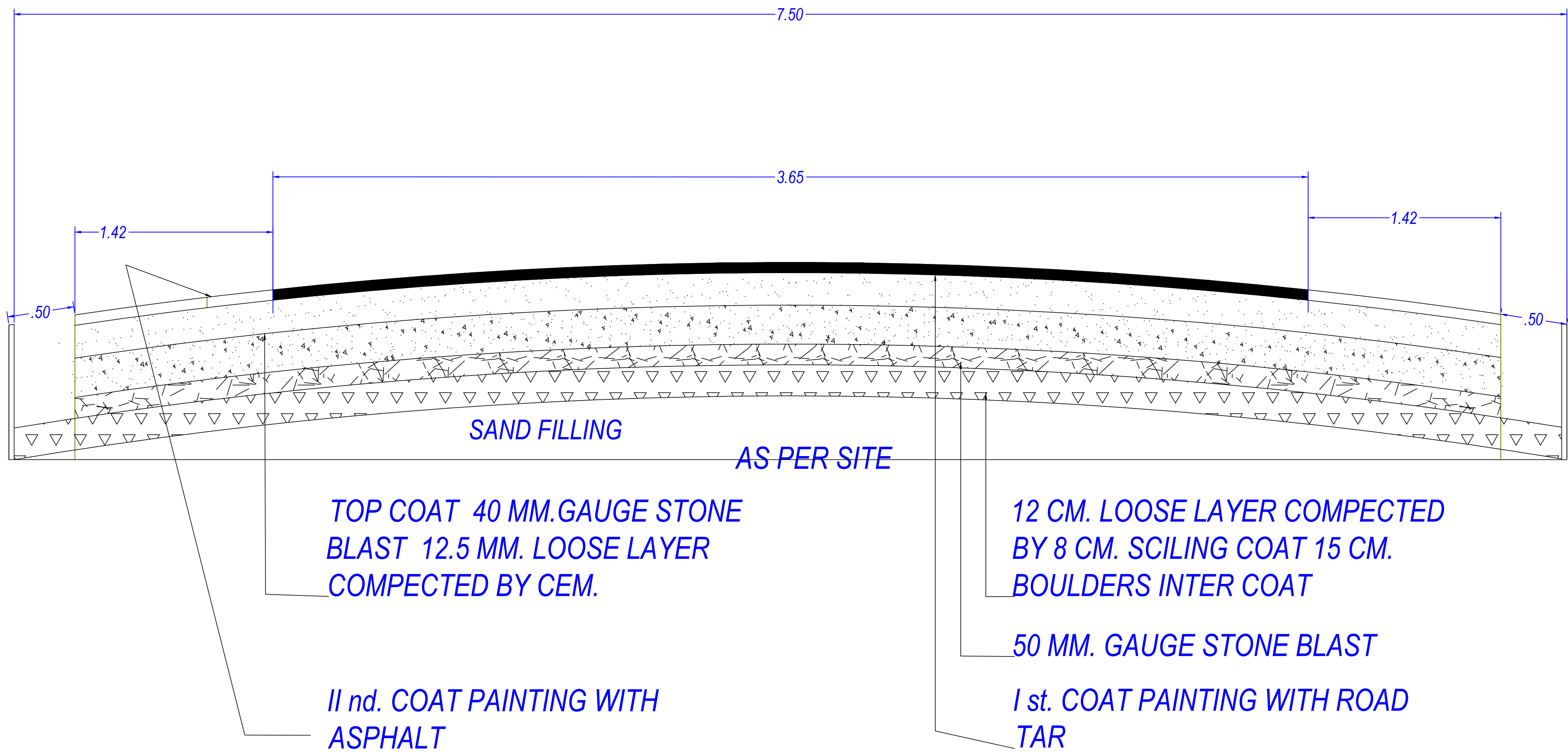
DETAIL OF ROAD SECTOIN SCALE:-N.T.S.
