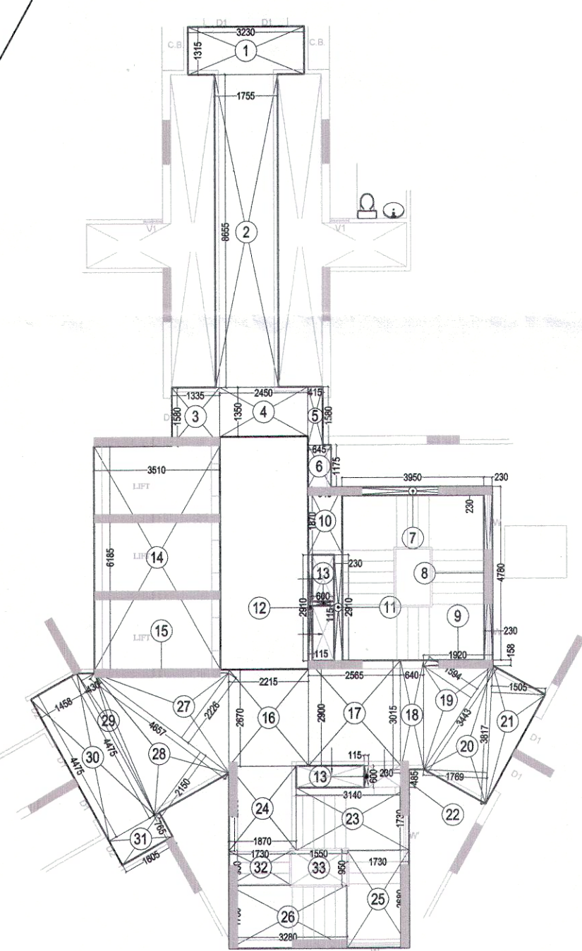
CIRCULATION F.A.R. AREA DETAIL OF GROUND FLOOR
