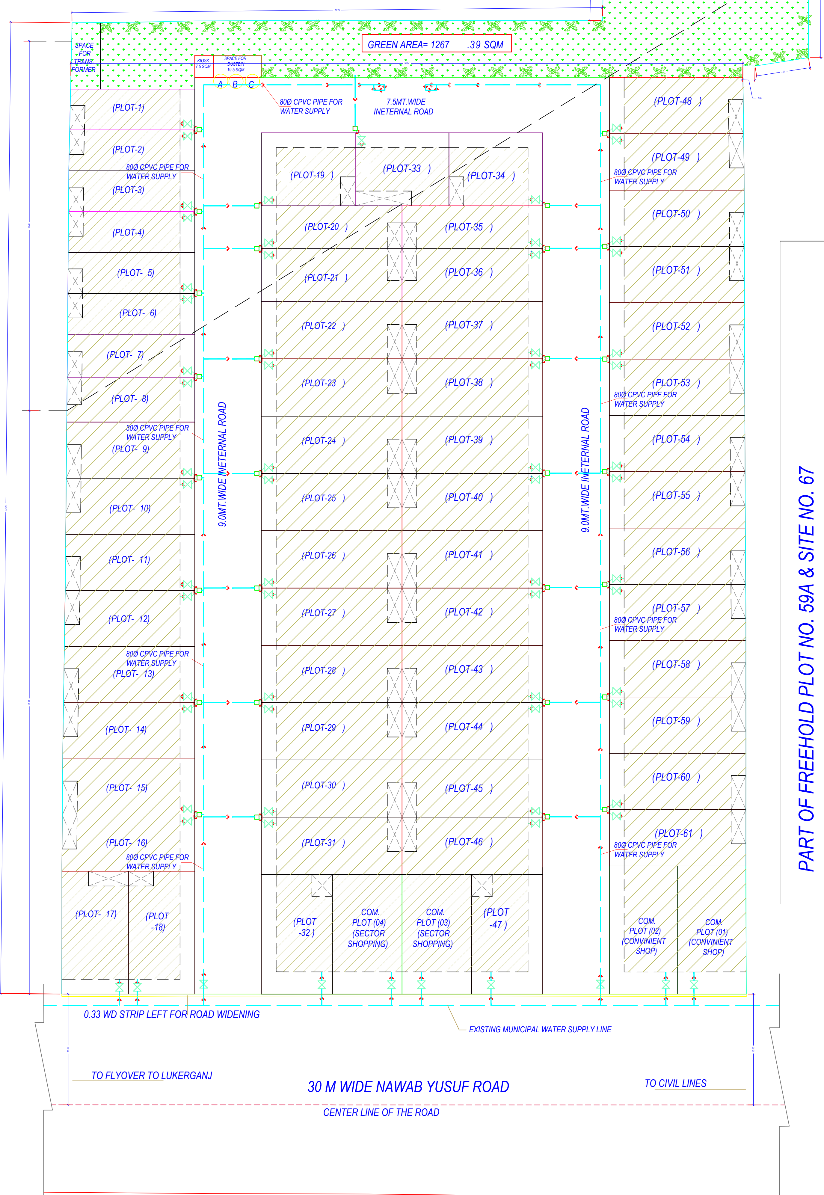
PROPOSED WATER SUPPLY LAYOUT PLAN
