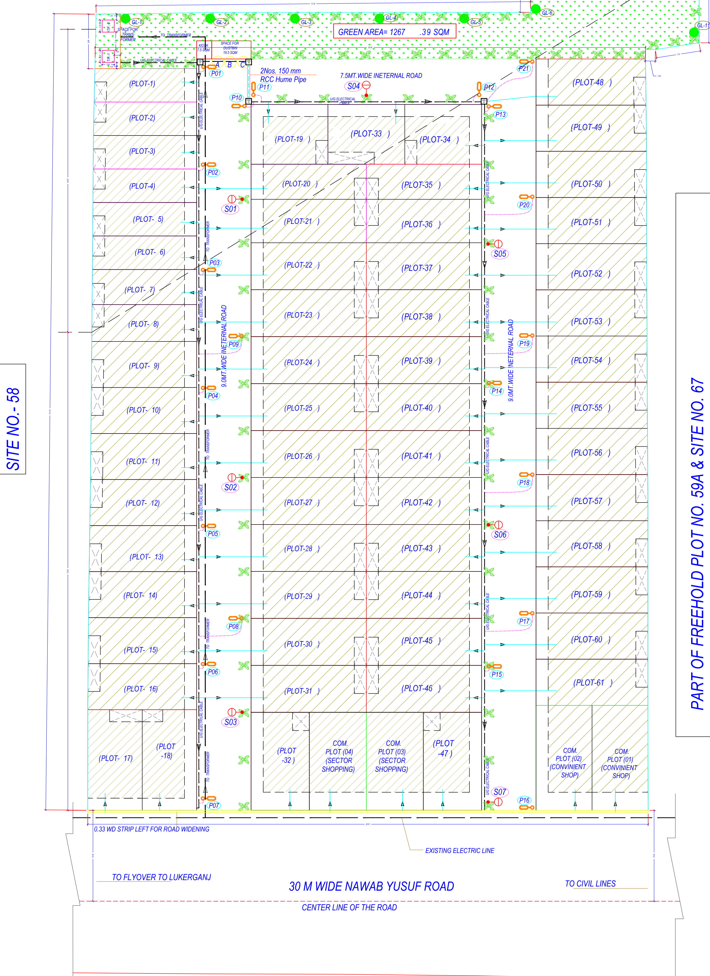
PROPOSED ELECTRIC LAYOUT PLAN
