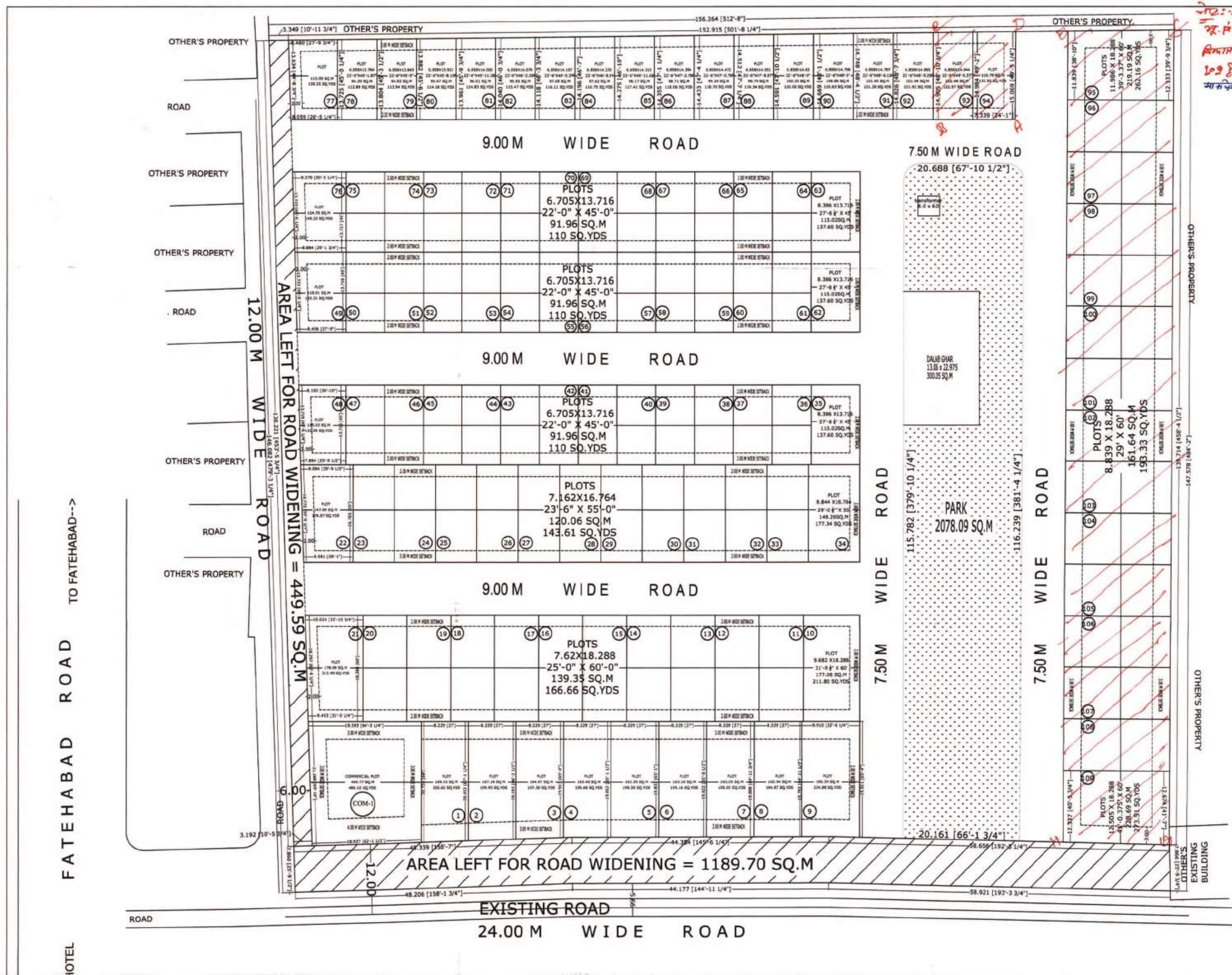
LAYOUT PLAN SCALE -:(1:400)
