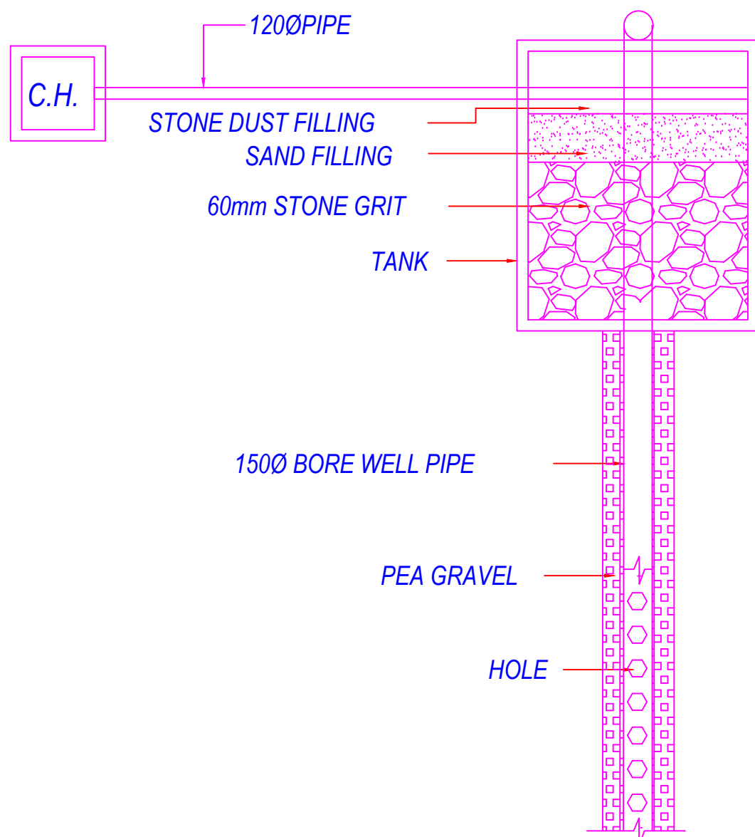
X-SECTION OF RAIN WATER HARVESTING PIT SCALE: N.T.S.
