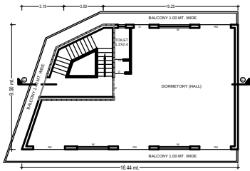
TYPICAL FIRST FL. & SECOND FLOOR PLAN
