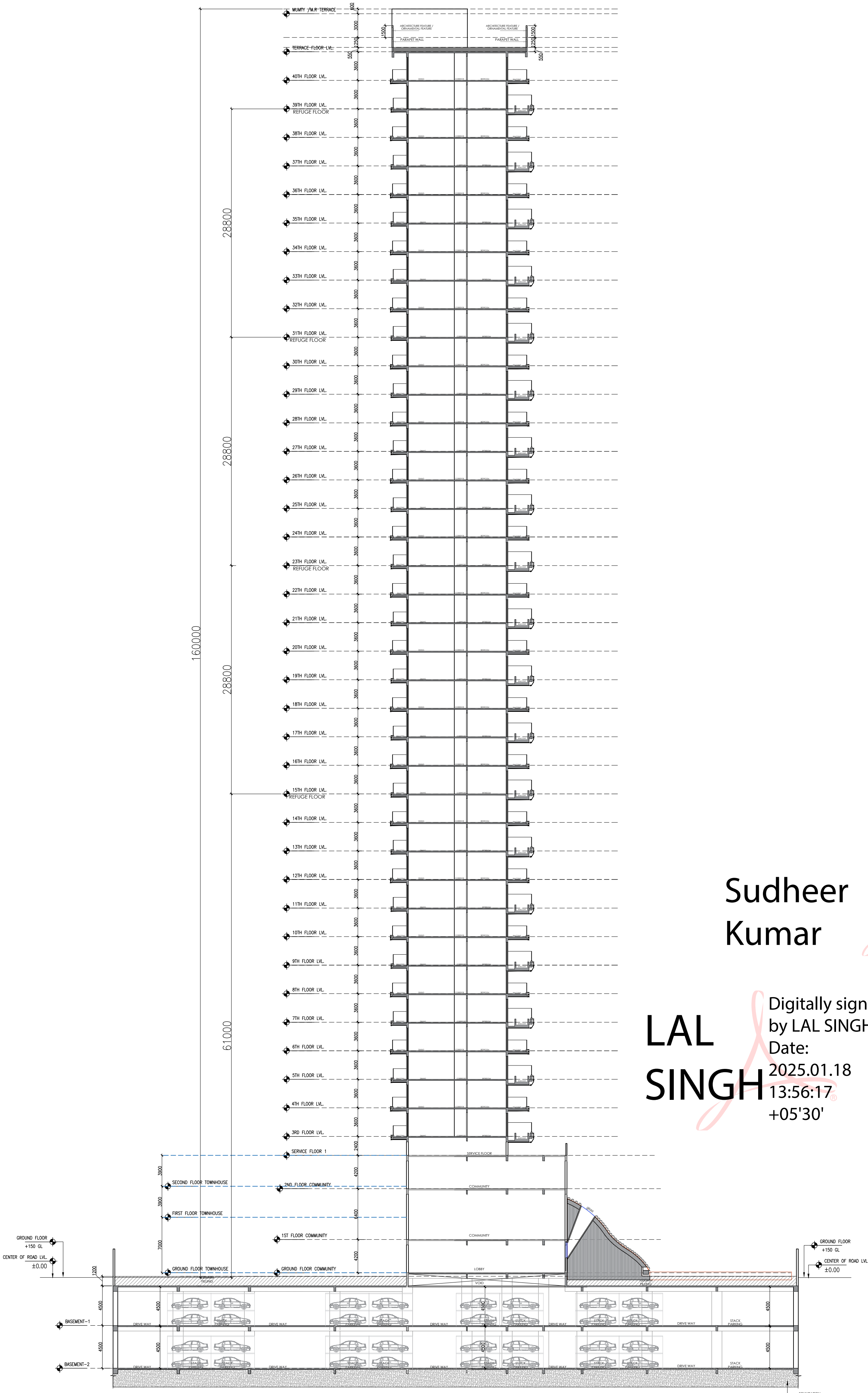
SECTION-9-9
