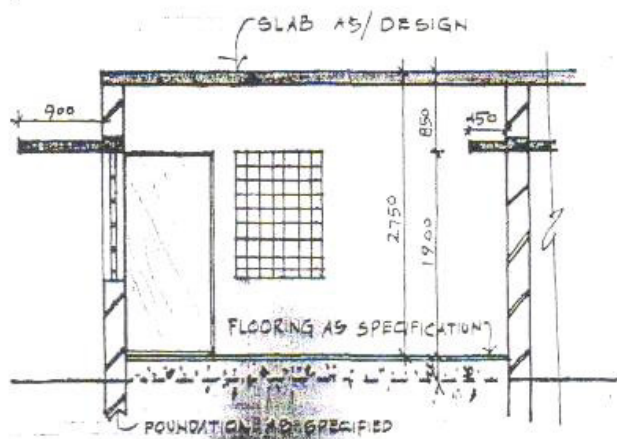
SECTION AT C-D
