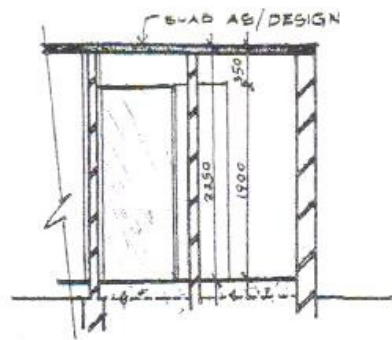
SECTION AT A-B
