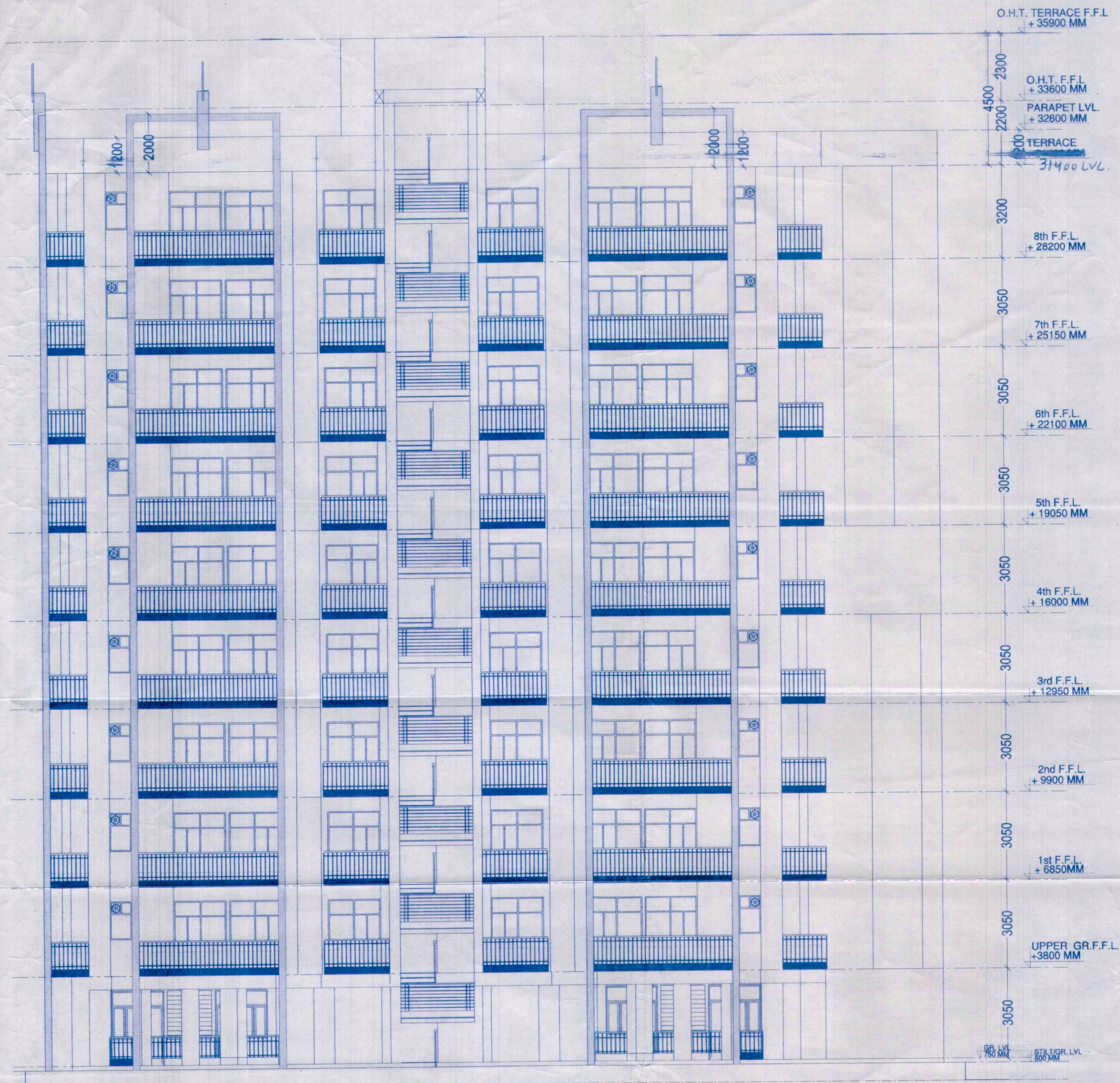
FRONT ELEVATION
