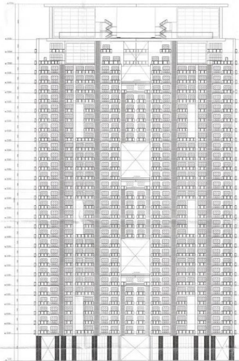
REAR(GOLF FACING) ELEVATION
