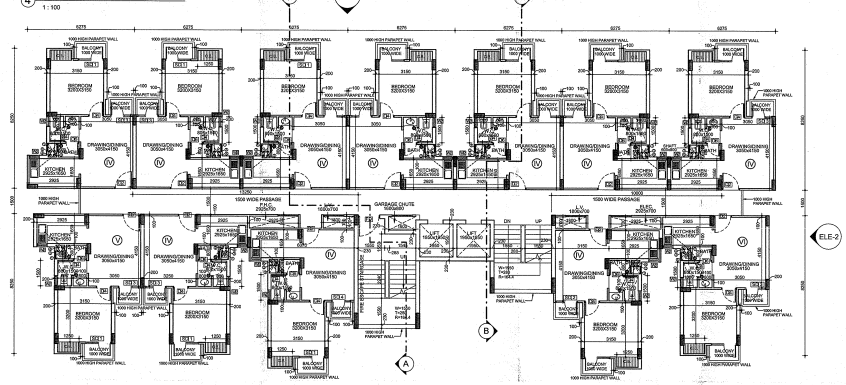
⑤ 13TH & 14TH FLOOR PLAN
