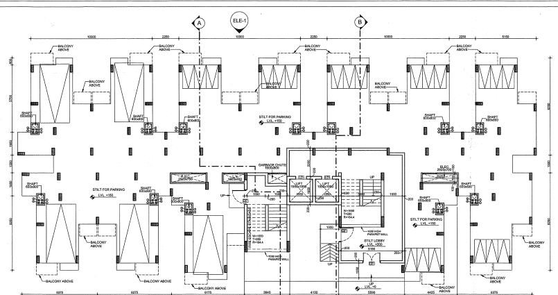
① STILT FLOOR PLAN 1:100
