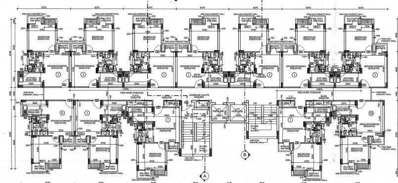
② 1ST TO 4TH FLOOR PLAN 1:100
