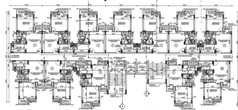
③ 5TH FLOOR PLAN 1:100
