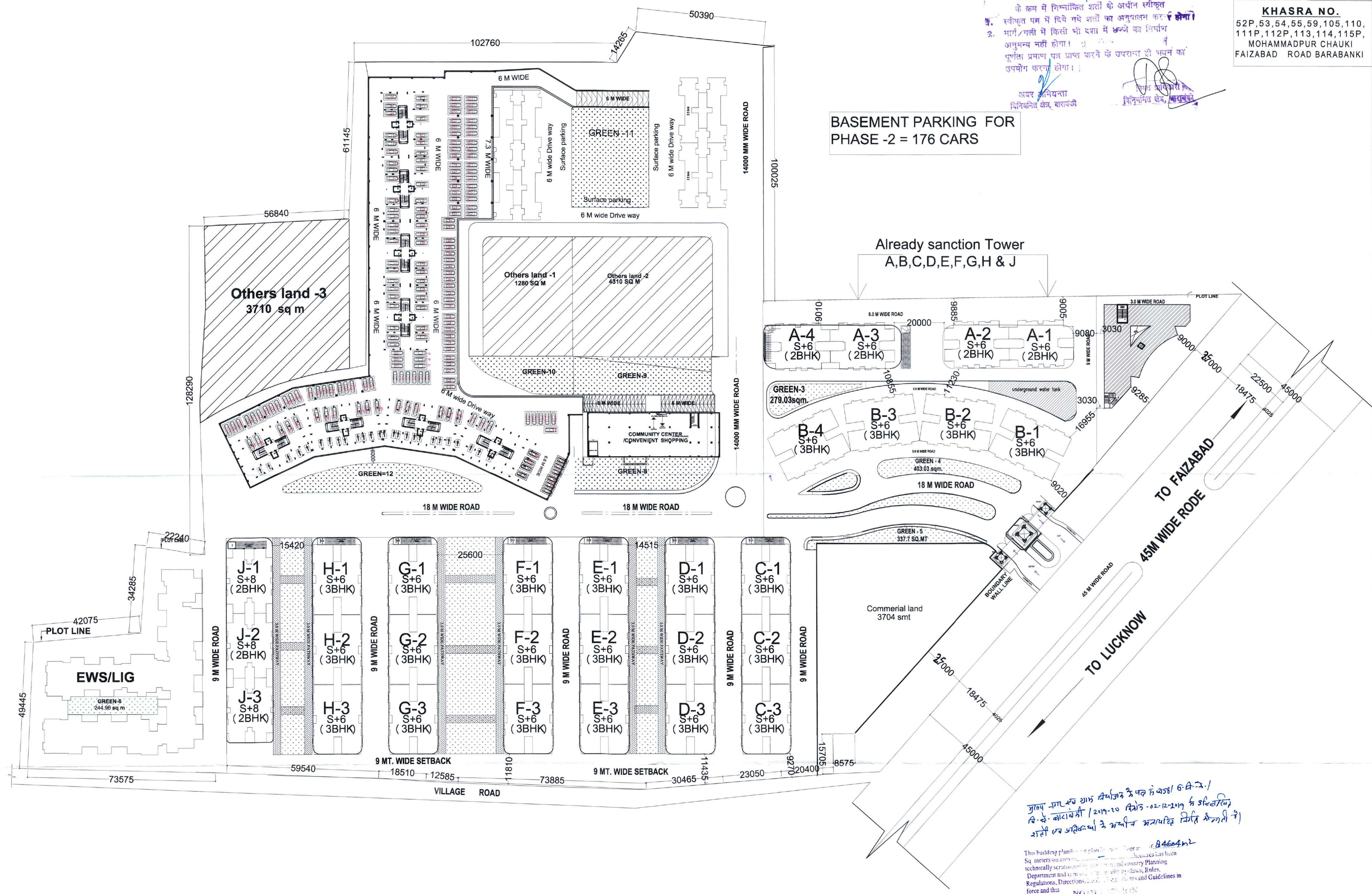
Basement Parking Layout SCALE:- 1:550
