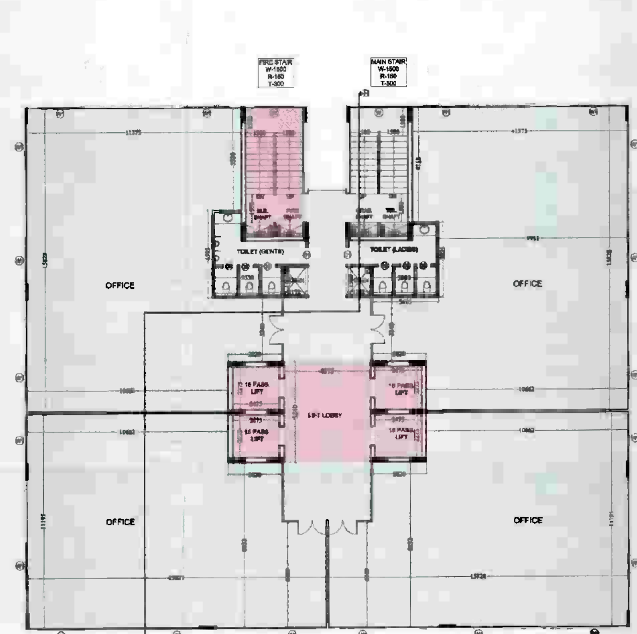
TOWER -B 8th. & 9th. FLOOR PLAN
