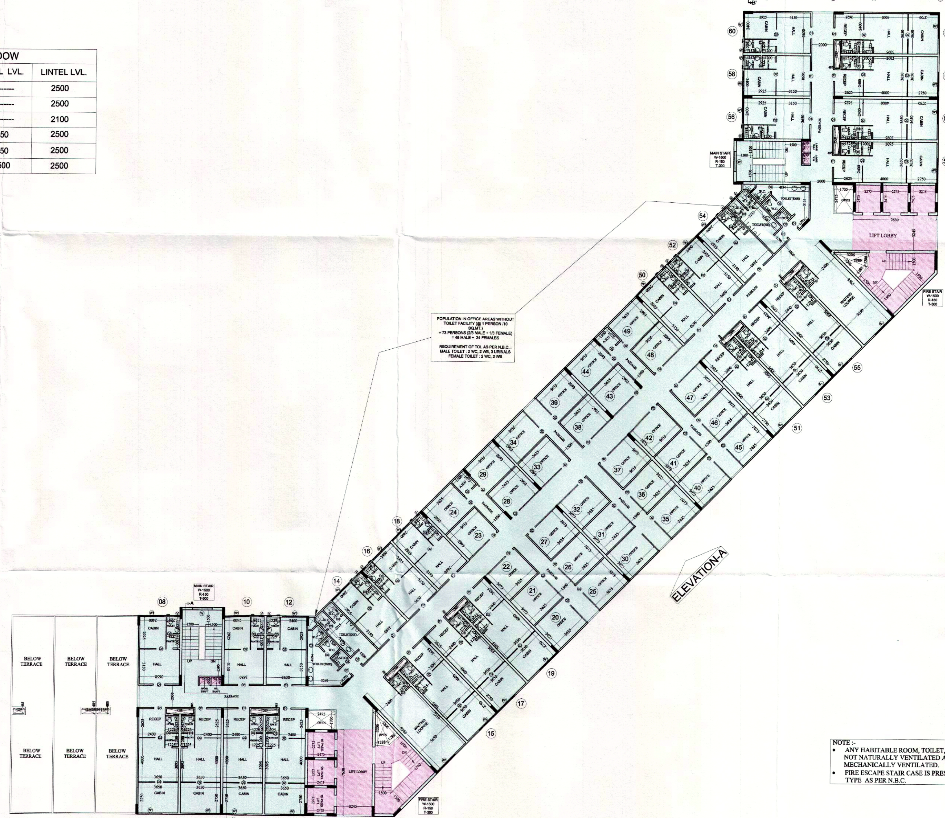
TOWER - A 12th. FLOOR PLAN
