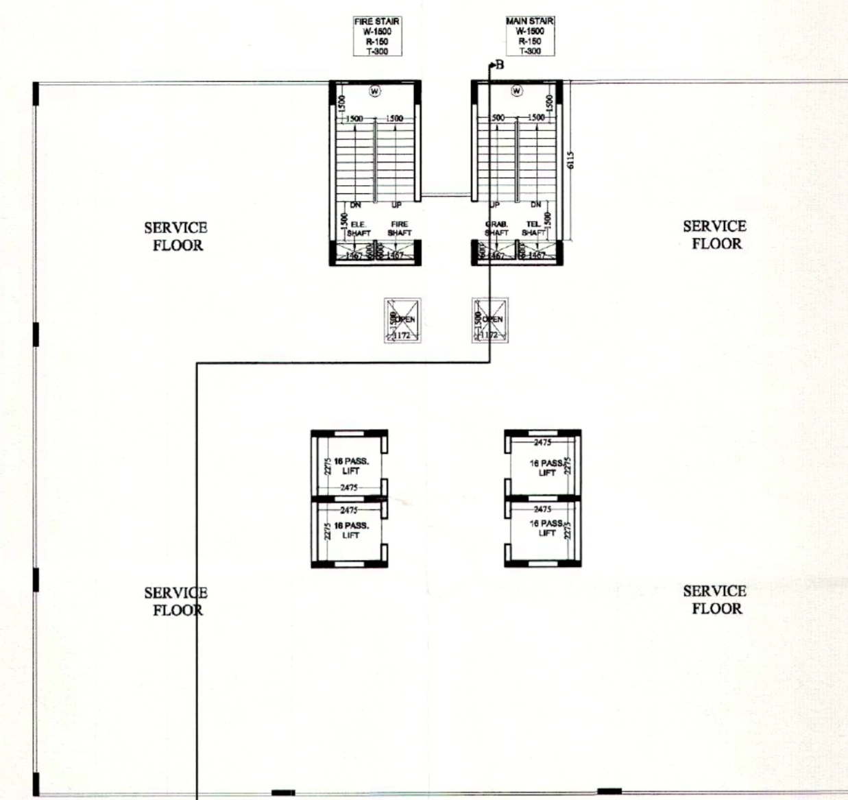
TOWER -B (SERVICE FLOOR) 13th. FLOOR PLAN
