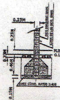
DETAIL OF RCC COLUMN
