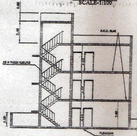
SECTION SCALE-1:100
