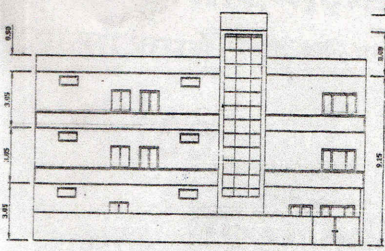
ELEVATION SCALE-1:100
