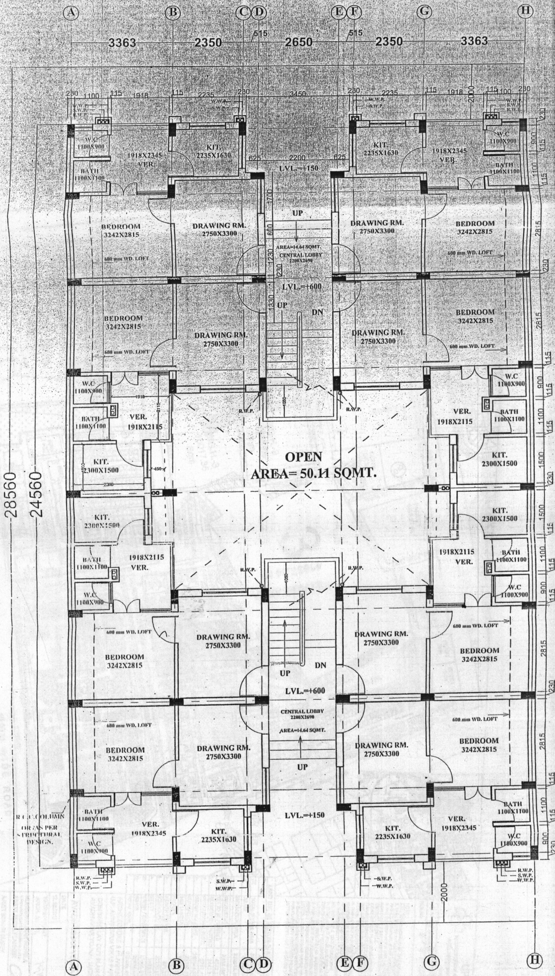
GROUND FLOOR PLAN (WORKING DRAWING)
