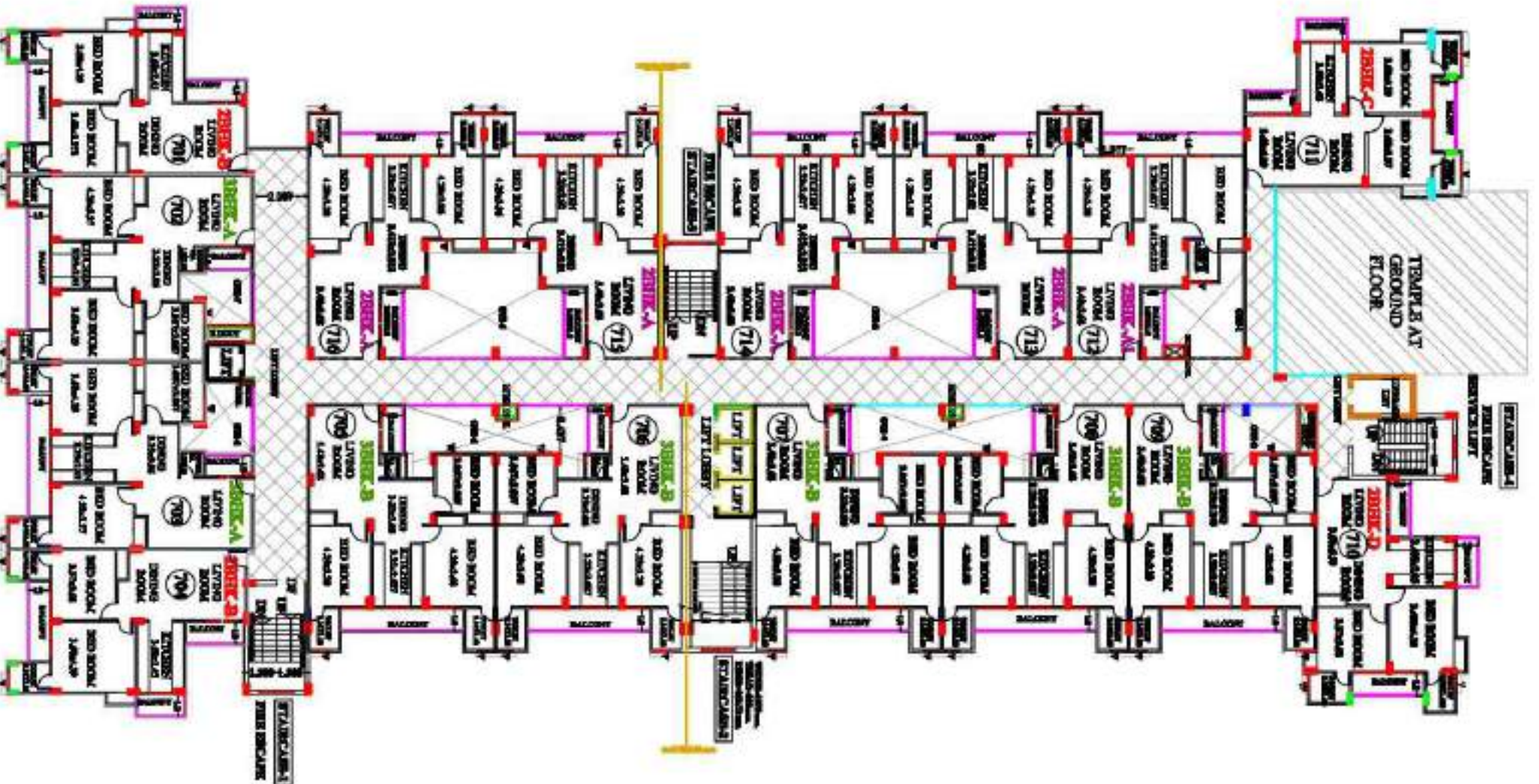
SEVENTH FLOOR PLAN
