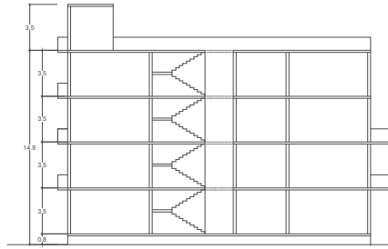
SECTION ELEVATION
