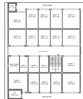
FIRST FLOOR PLAN AREA IN FAR 423.29 SQ.MT
