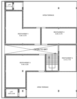
THIRD FLOOR PLAN AREA IN FAR 216.10 SQ.MT
