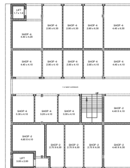
GROUND FLOOR PLAN AREA IN FAR 398.00 SQ.MT BUILD AREA 398.00 SQ.MT
