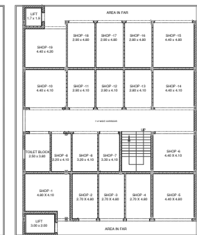
SECOND FLOOR PLAN AREA IN FAR 388.82 SQ.MT
