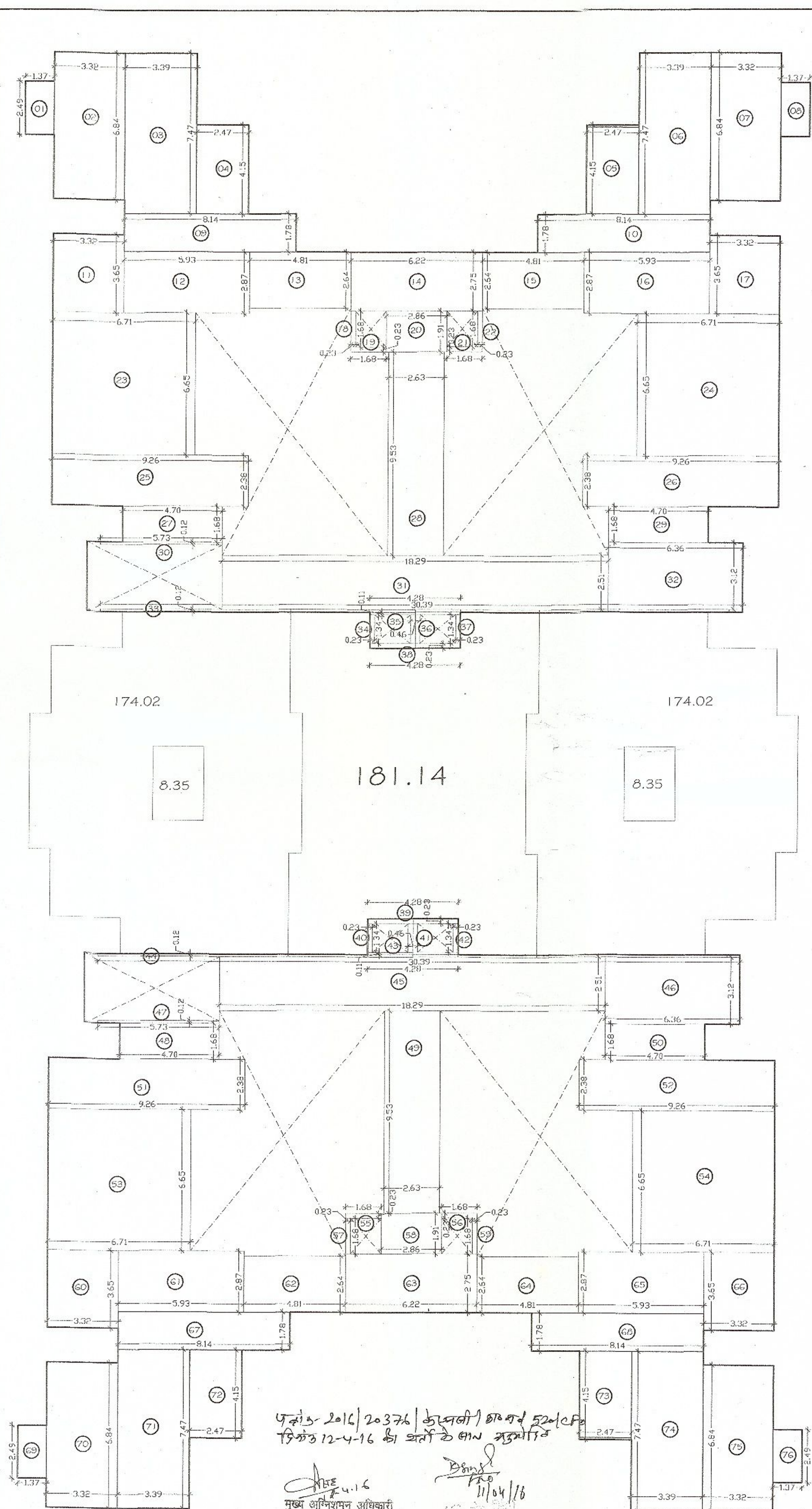
NINTH FLOOR PLAN
