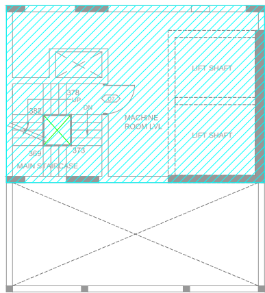
MACHINE ROOM LEVEL PLAN
