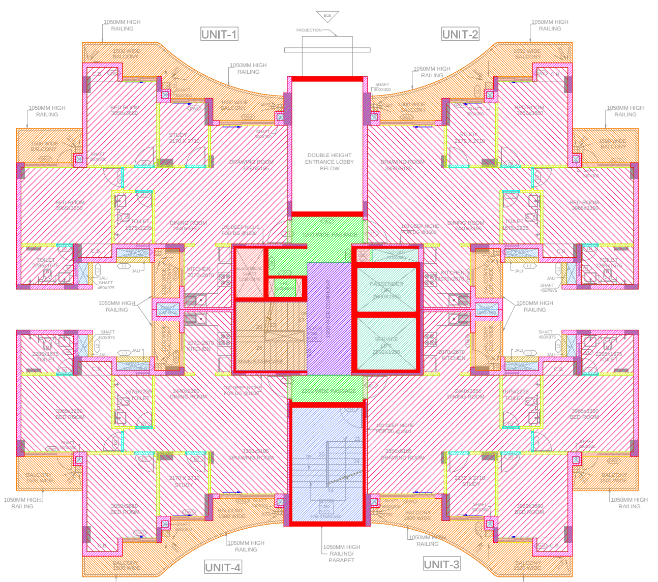
TOWER-A,B,C,D,E 1ST FLOOR PLAN
