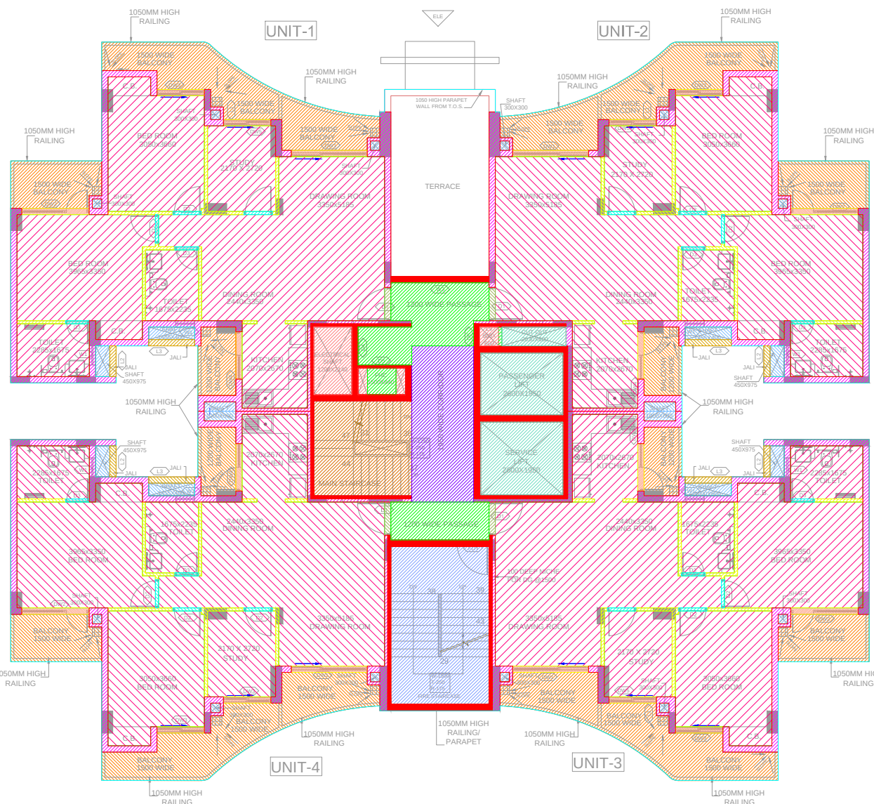
TOWER-A,B,C,D,E 2ND FLOOR TO 6TH FLOOR PLAN
