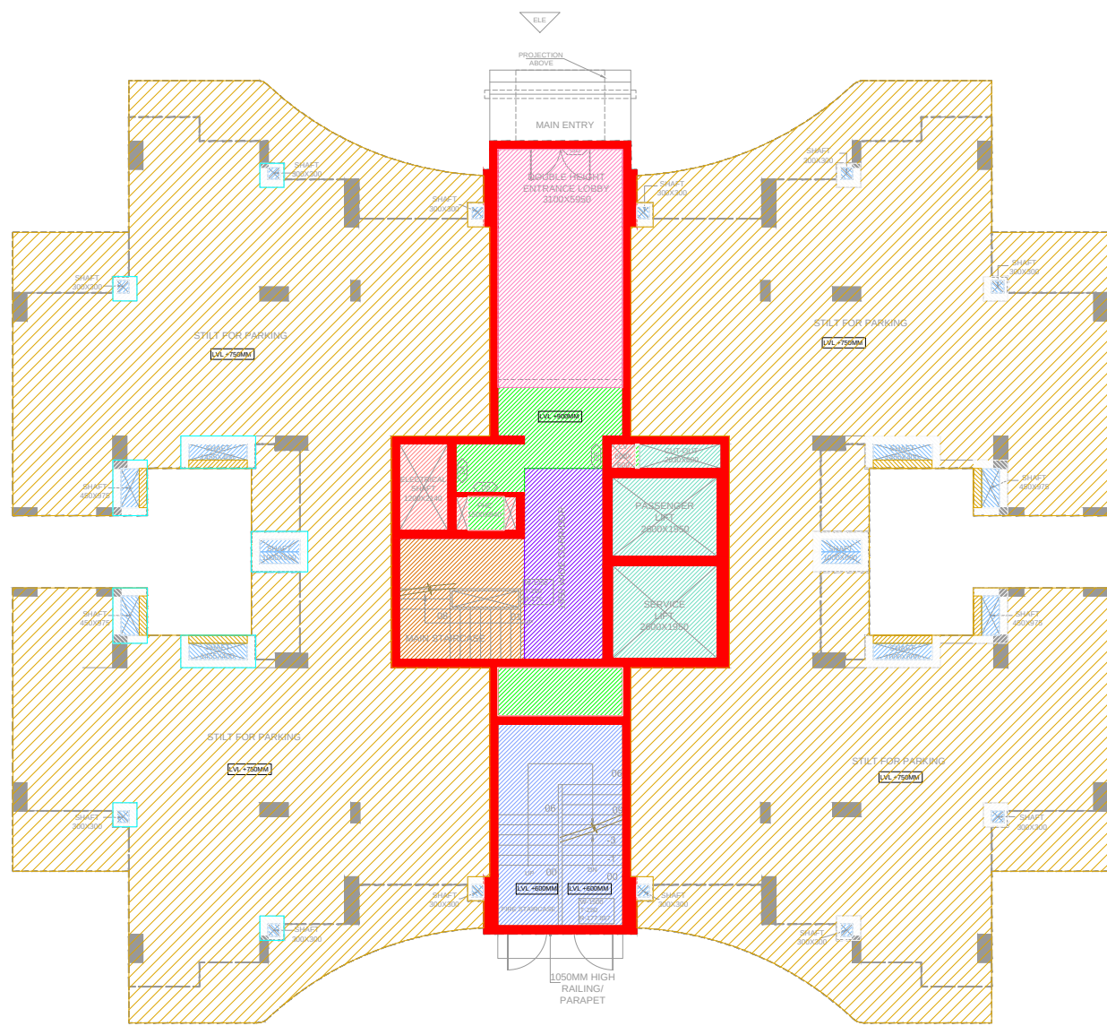
TOWER-A STILT FLOOR PLAN
