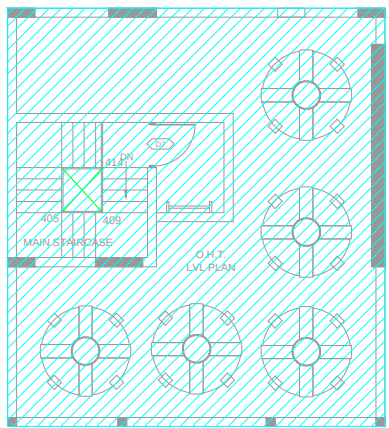
WATER TANK LEVEL PLAN
