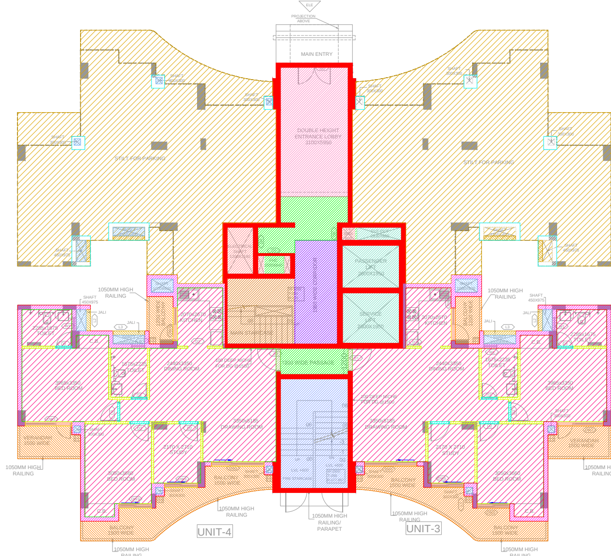
TOWER- B, C, D & E STILT FLOOR PLAN
