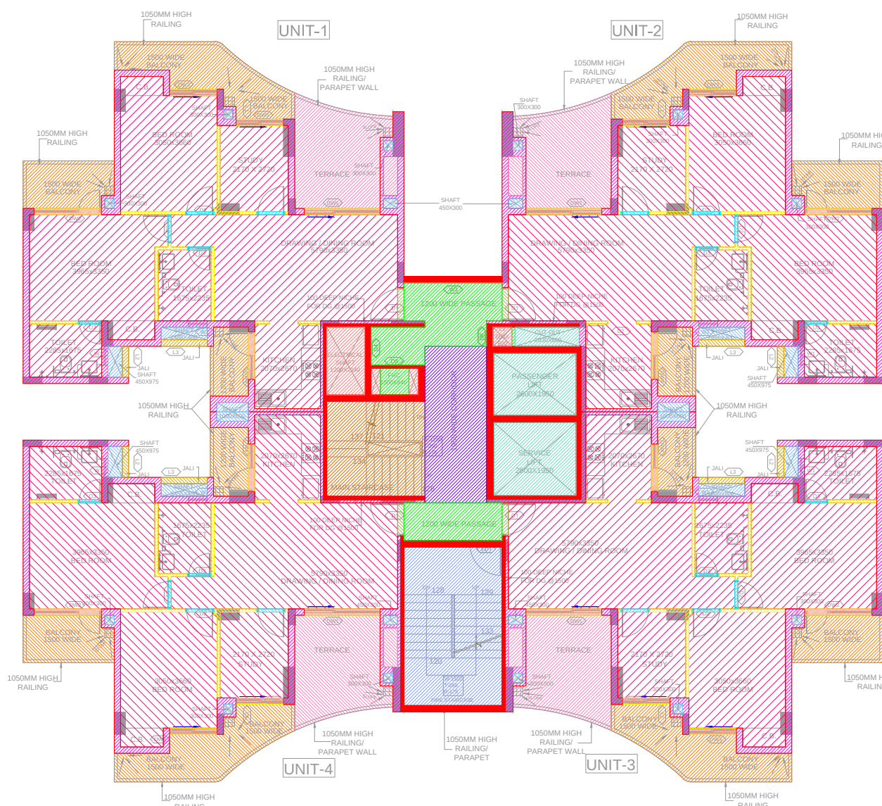
TOWER-A,B,C,D,E 7TH FLOOR PLAN
