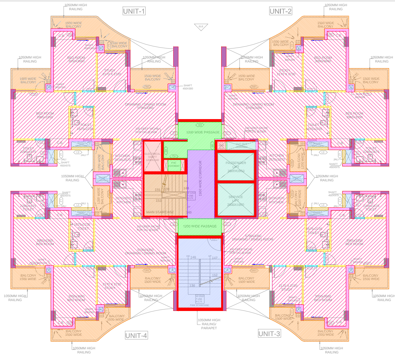
8TH TO 19TH FLOOR PLAN TOWER-A,B & C 8TH TO 18TH FLOOR PLAN TOWER- D & E
