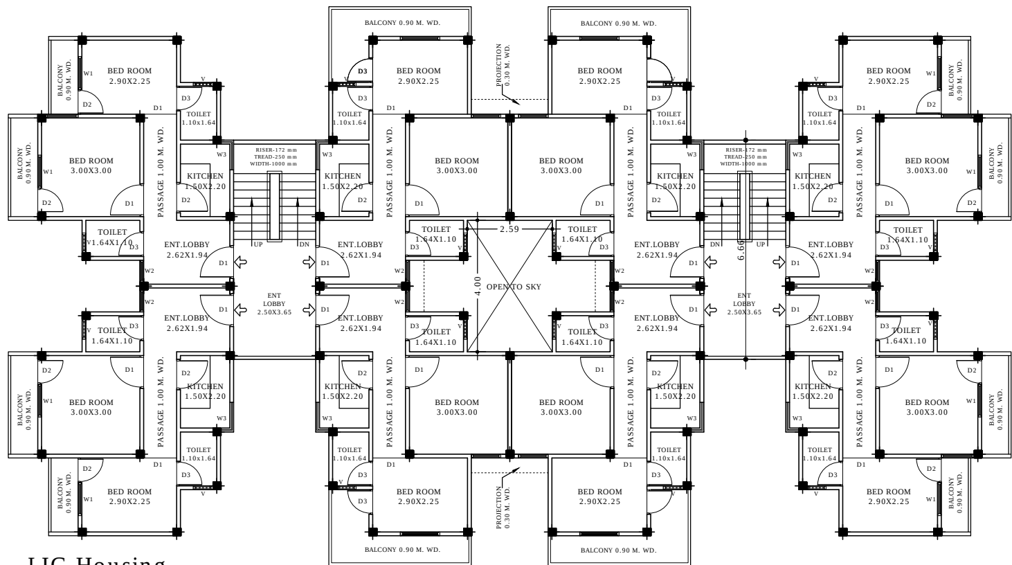
LIG Housing Typical Floor Plan
