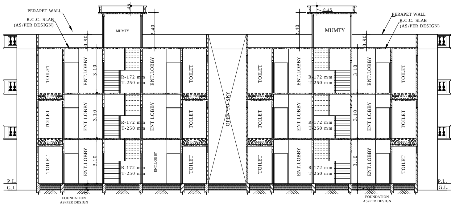
SECTION AT - A, B (L.I.G. HOUSES)
