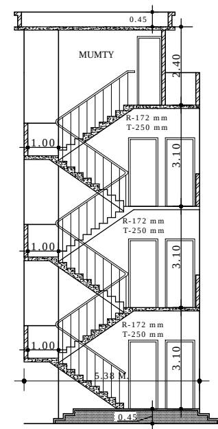
E.W.S.HOUSES STAIR DETAIL
