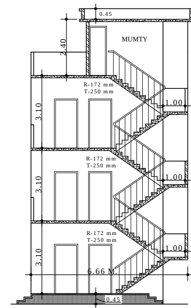
L.I.G.HOUSES STAIR DETAIL
