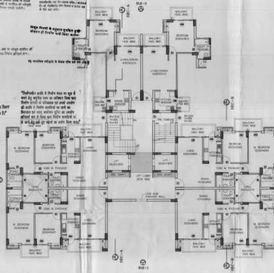
PROPOSED 12TH TO 18TH FLOOR PLAN (FOR TOWER-74) PROPOSED 12TH TO 18TH FLOOR PLAN (FOR TOWER-75)
