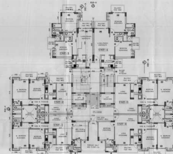
TYPICAL FLOOR PLAN 2ND TO 17TH FLOOR (FOR TOWER-T1) 2ND TO 18TH FLOOR (FOR TOWER-T3) 2ND TO 7TH FLOOR (FOR TOWER-T4) 2ND TO 6TH FLOOR (FOR TOWER-T5)
