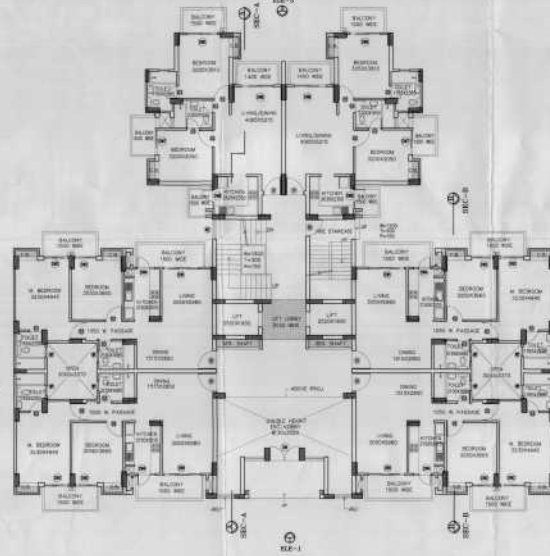
GROUND FLOOR PLAN- T-74 & T-5
