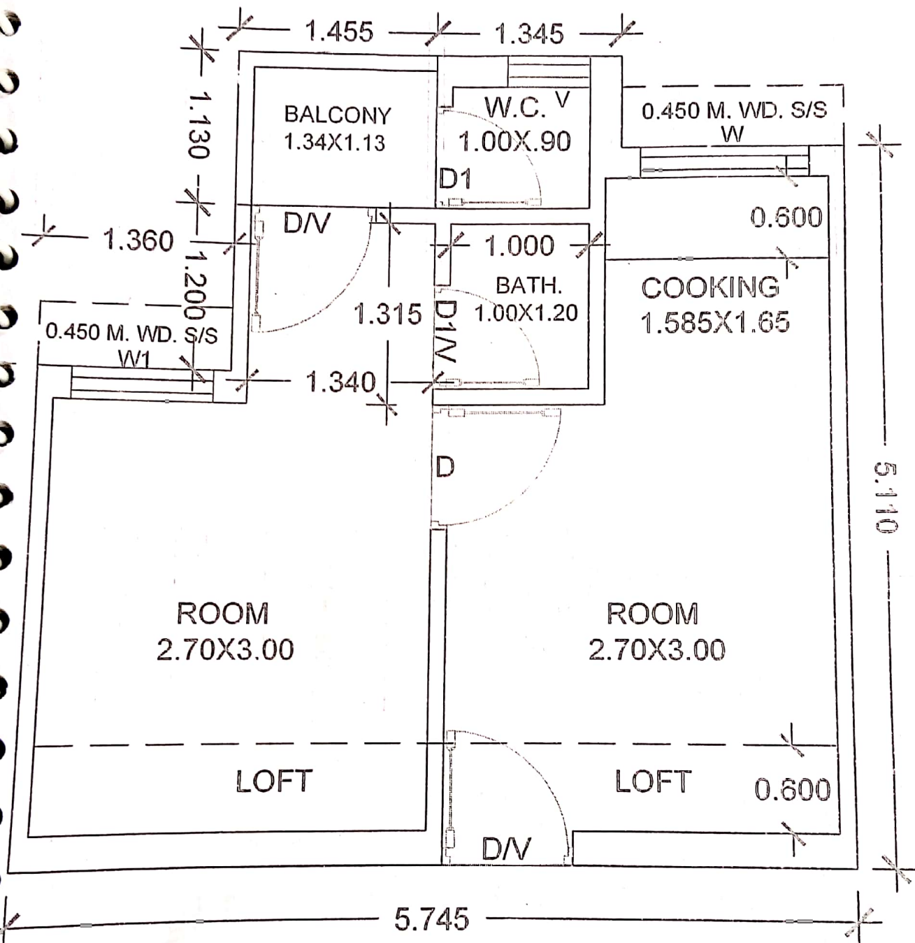
UNIT PLAN
