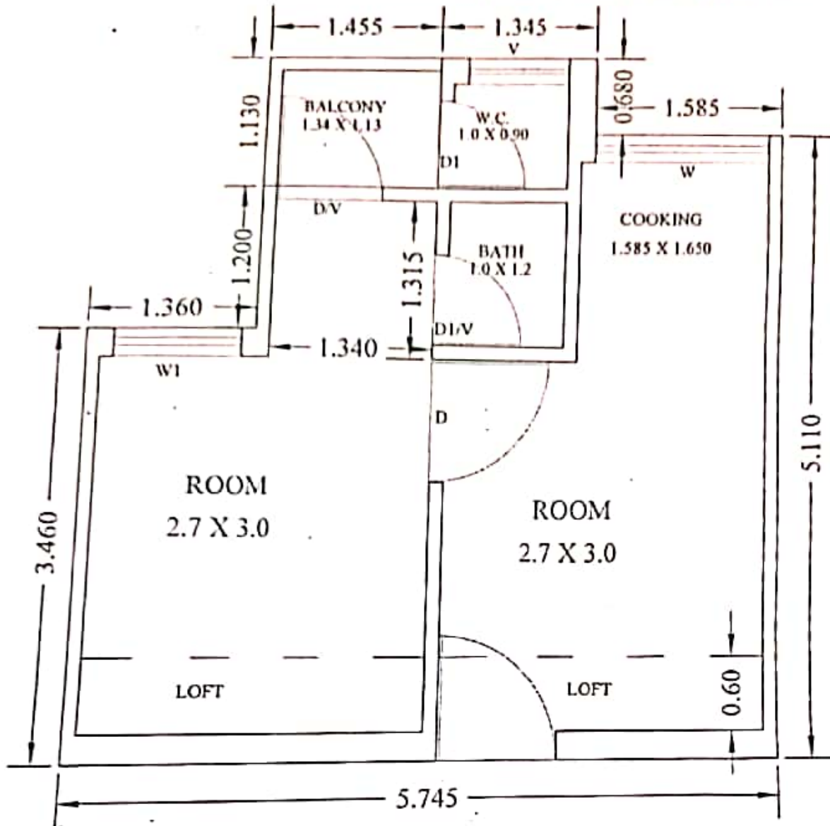
UNIT PLAN
