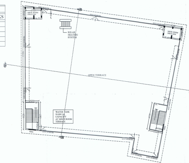
TERRACE PLAN
