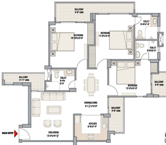
TYPE-III (3 B/R)
