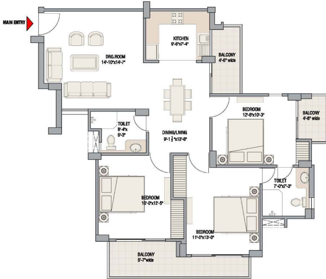
TYPE-II (3 B/R)
