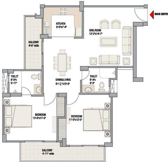
TYPE-I (2 B/R)
