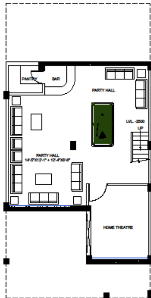
BASEMENT PLAN
