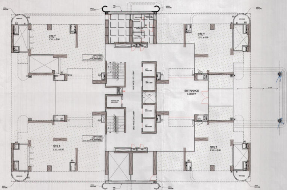
3 B.H.K. SMALL STILT LEVEL PLAN
