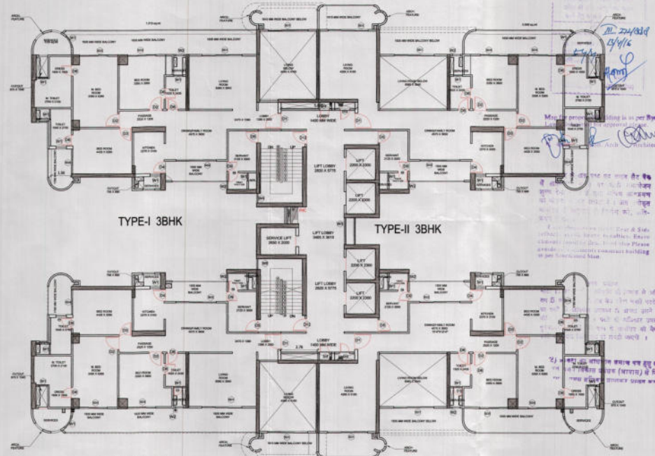
30th FLOOR PLAN (3 BHK SMALL)
