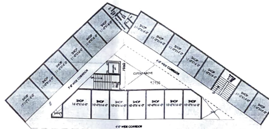
FIRST & SECOND FLOOR PLAN
