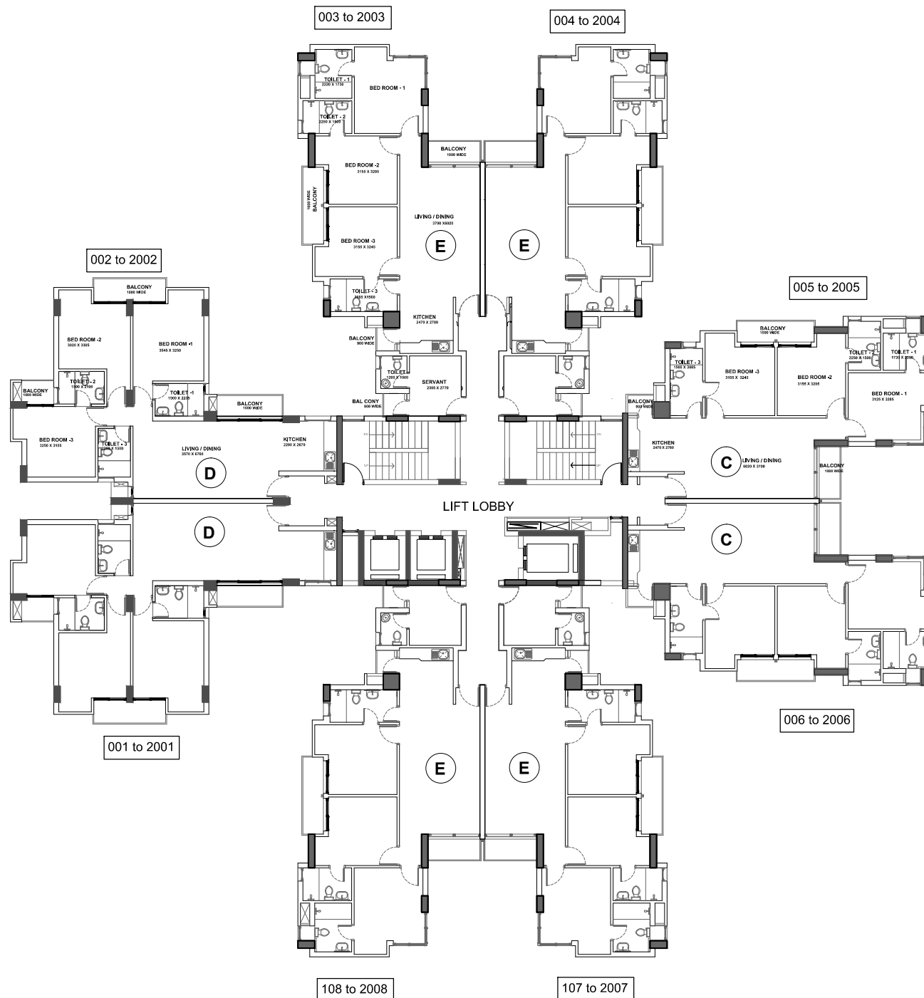
TYPICAL FLOOR PLAN - 3BHK
