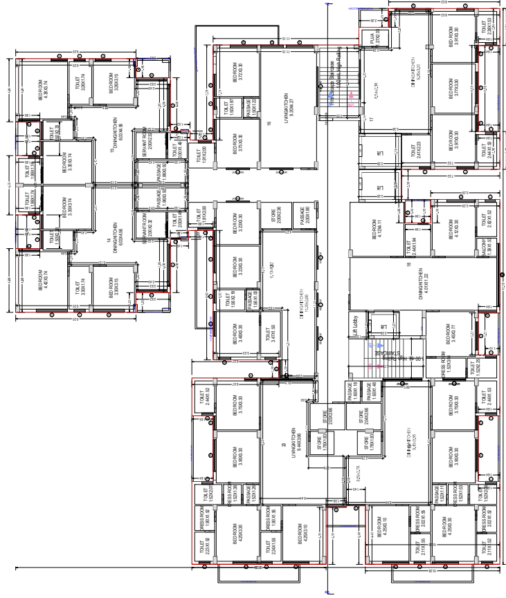
TYPICAL - 2-3 FLOOR PLAN (Proposed) (SCALE 1:100)
