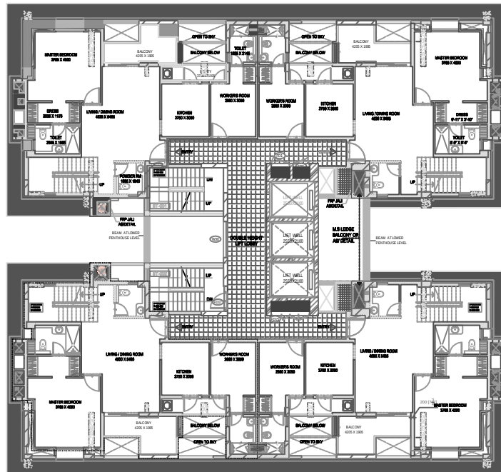
LOWER PENTHOUSE
