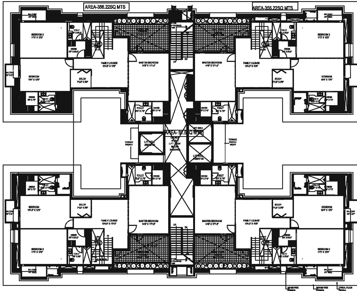
UPPER PENTHOUSE PLAN
