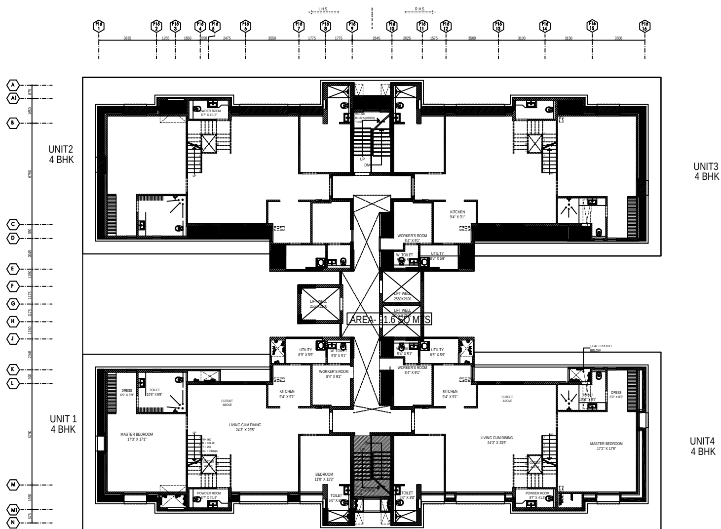
LOWER PENTHOUSE PLAN
