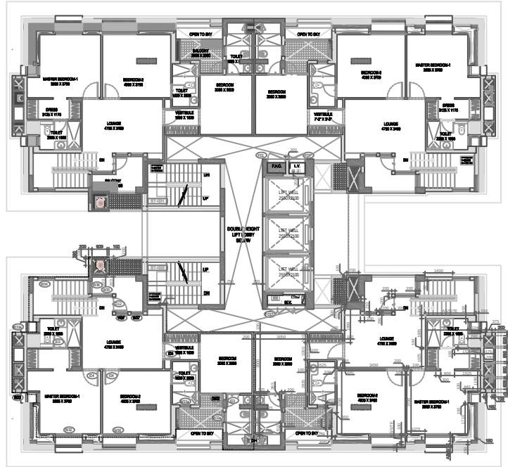
UPPER PENTHOUSE
