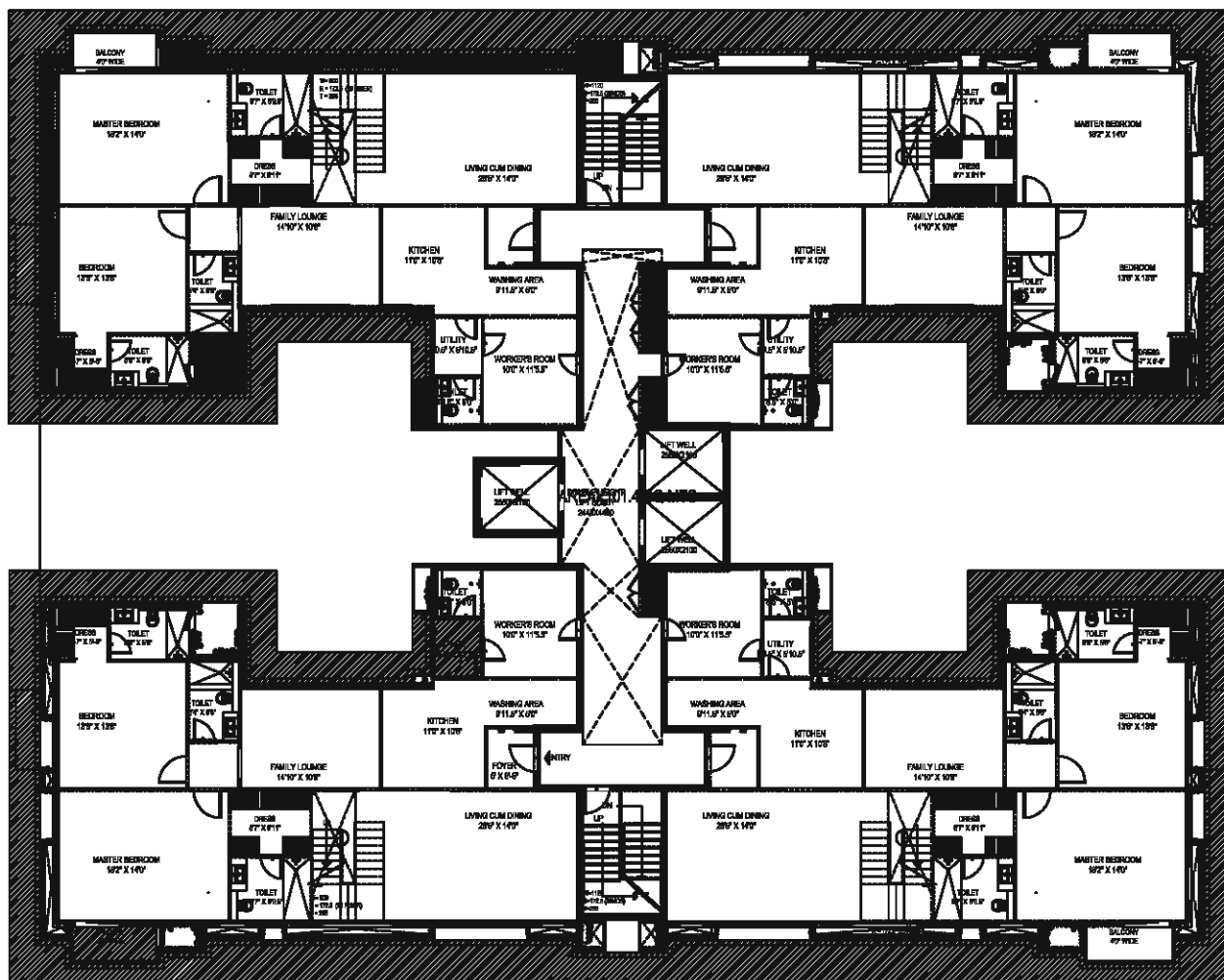
LOWER PENTHOUSE PLAN
