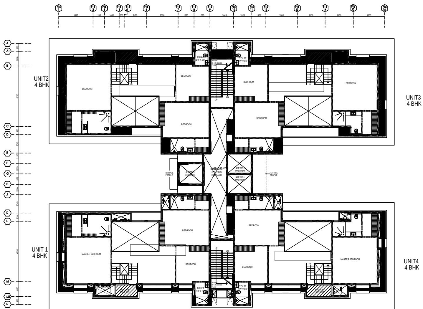
UPPER PENTHOUSE PLAN
