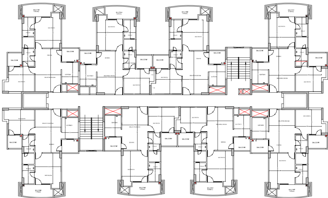
TOWER-C6 TYPICAL FLOOR PLAN
