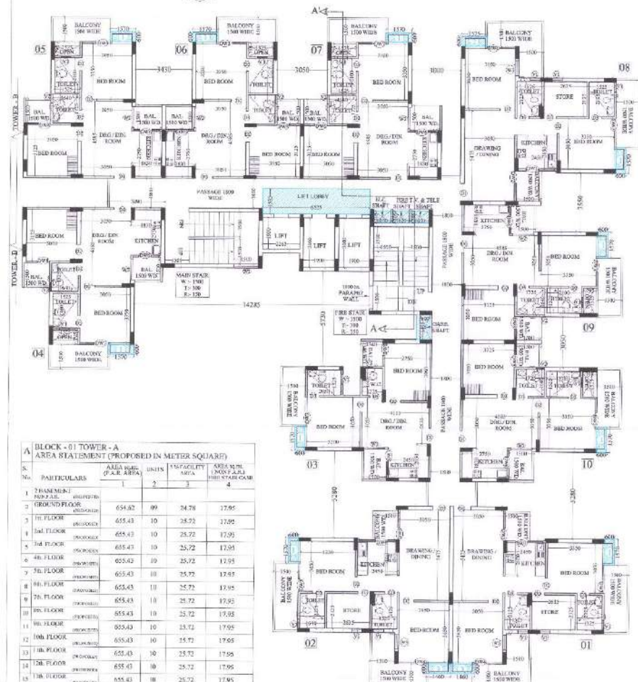
BLOCK - 01 TOWER - A 2nd. TO 23rd. FLOOR PLAN
