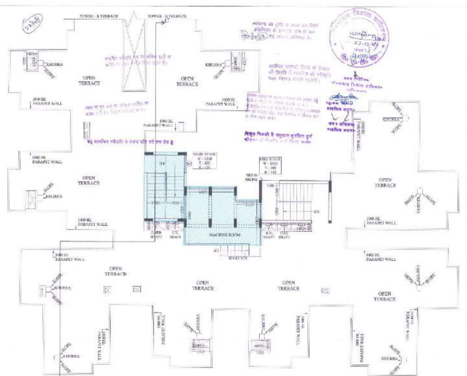
BLOCK - 1 (TOWER - C) TERRACE PLAN
