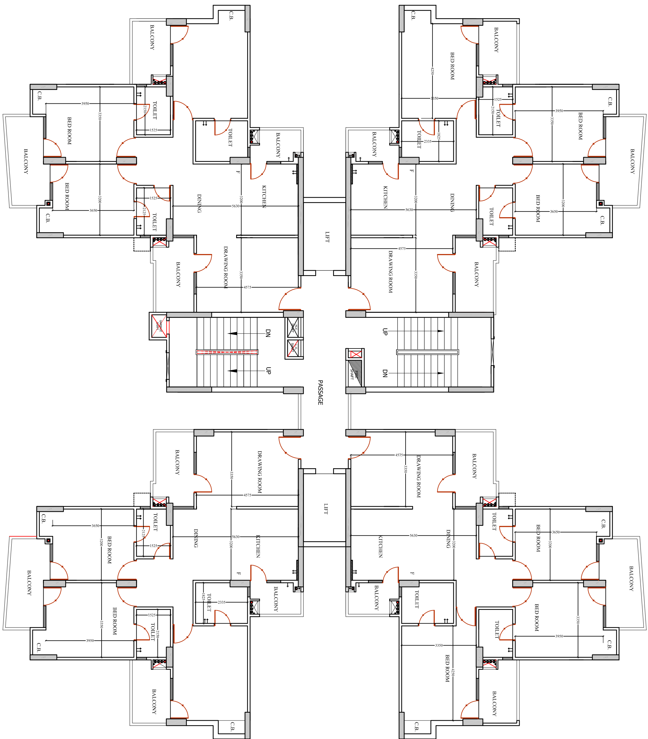
TOWER-E7 TYPICAL FLOOR PLAN
