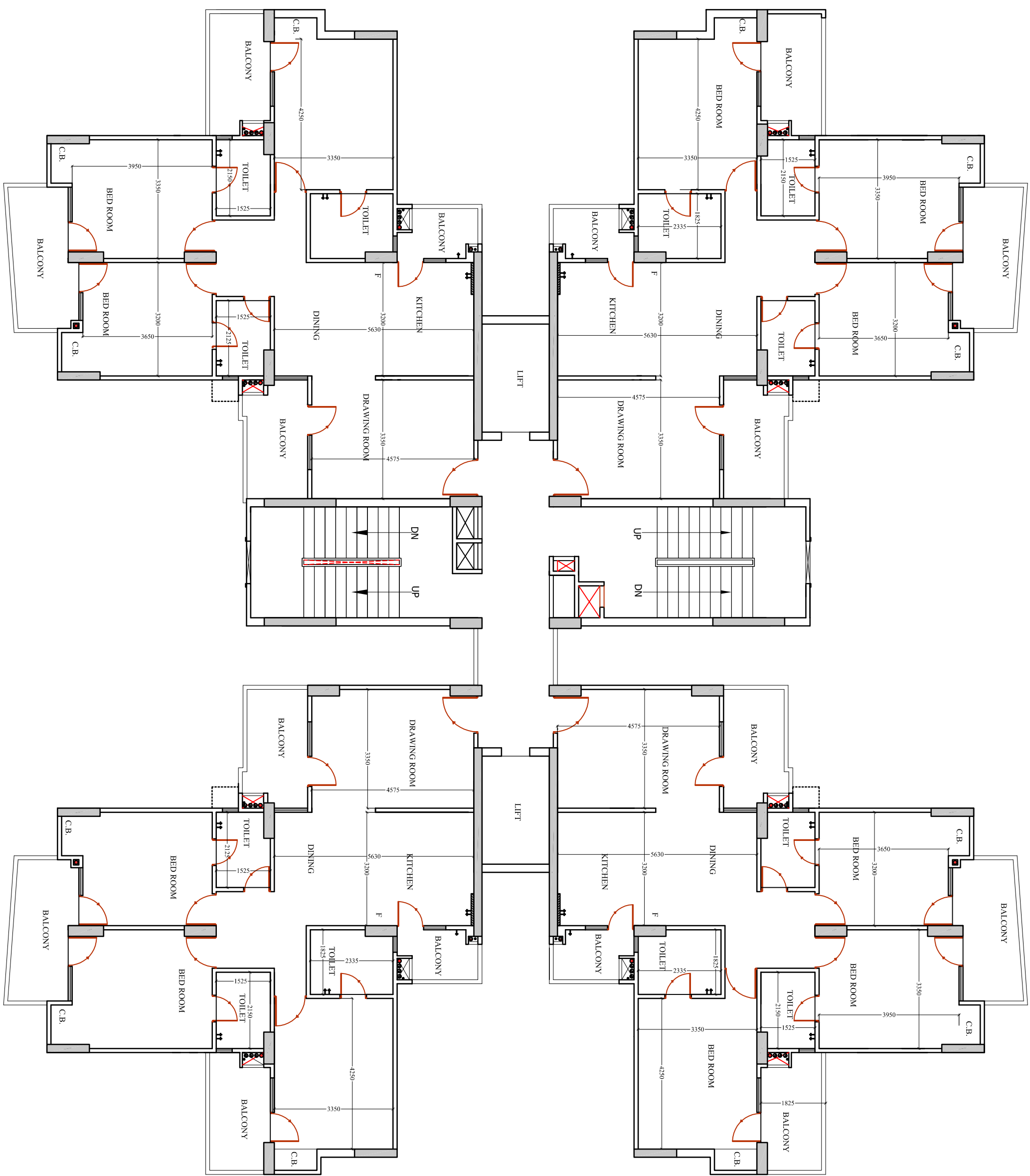
TOWER-E6 TYPICAL FLOOR PLAN
