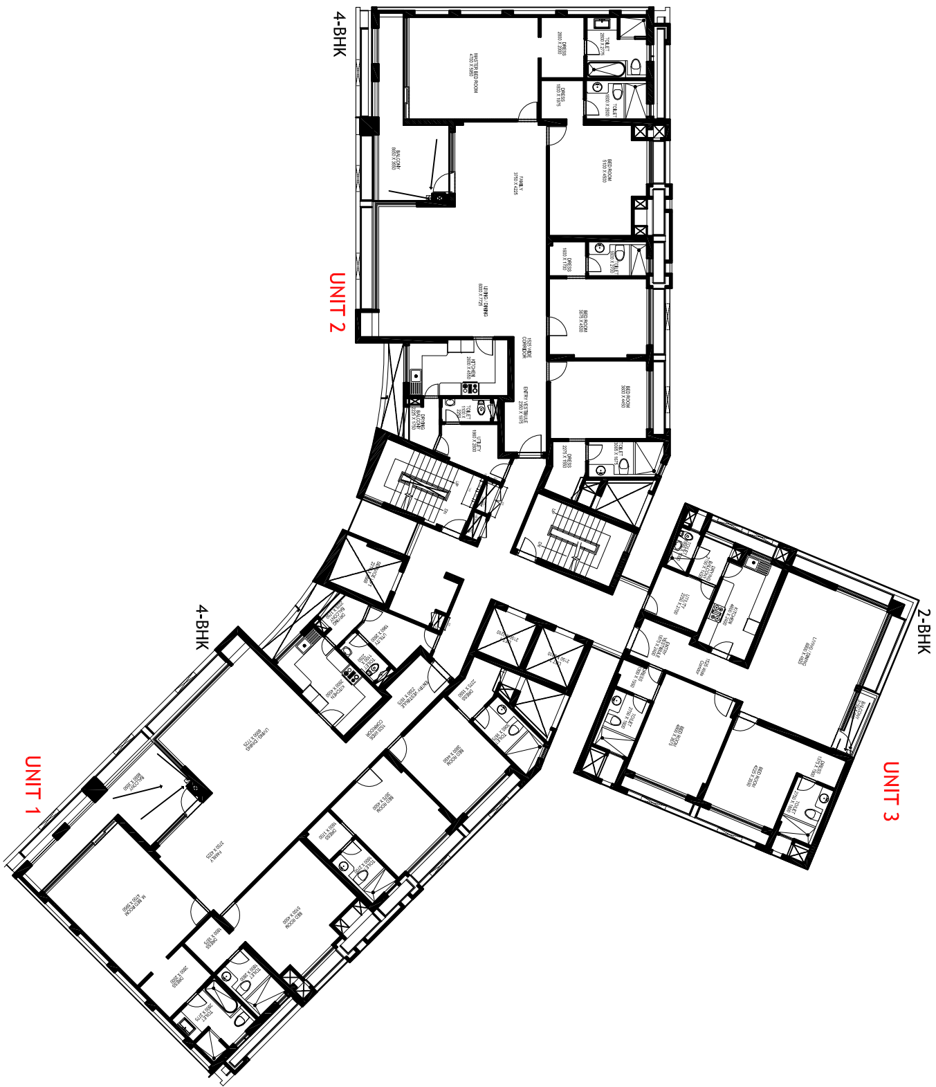
KALYPSO COURT-TOWER 7&8-3rd, 11th & 19th FLOOR PLAN
