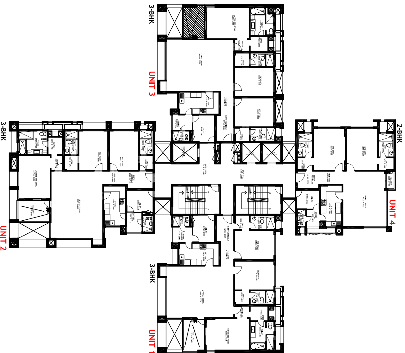
KALYPSO COURT-TOWER 10-2nd,7th,8th,9th,10th,15th
