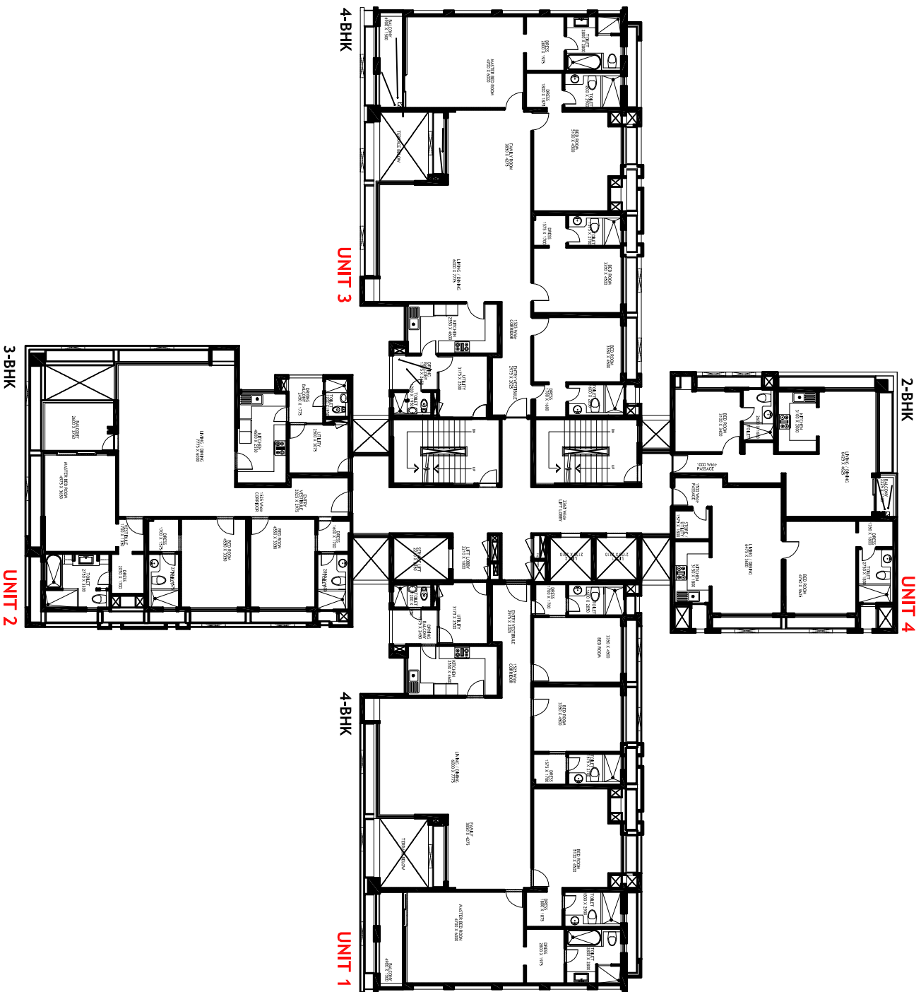
KALYPSO COURT-TOWER 9-4th & 12th FLOOR PLAN
