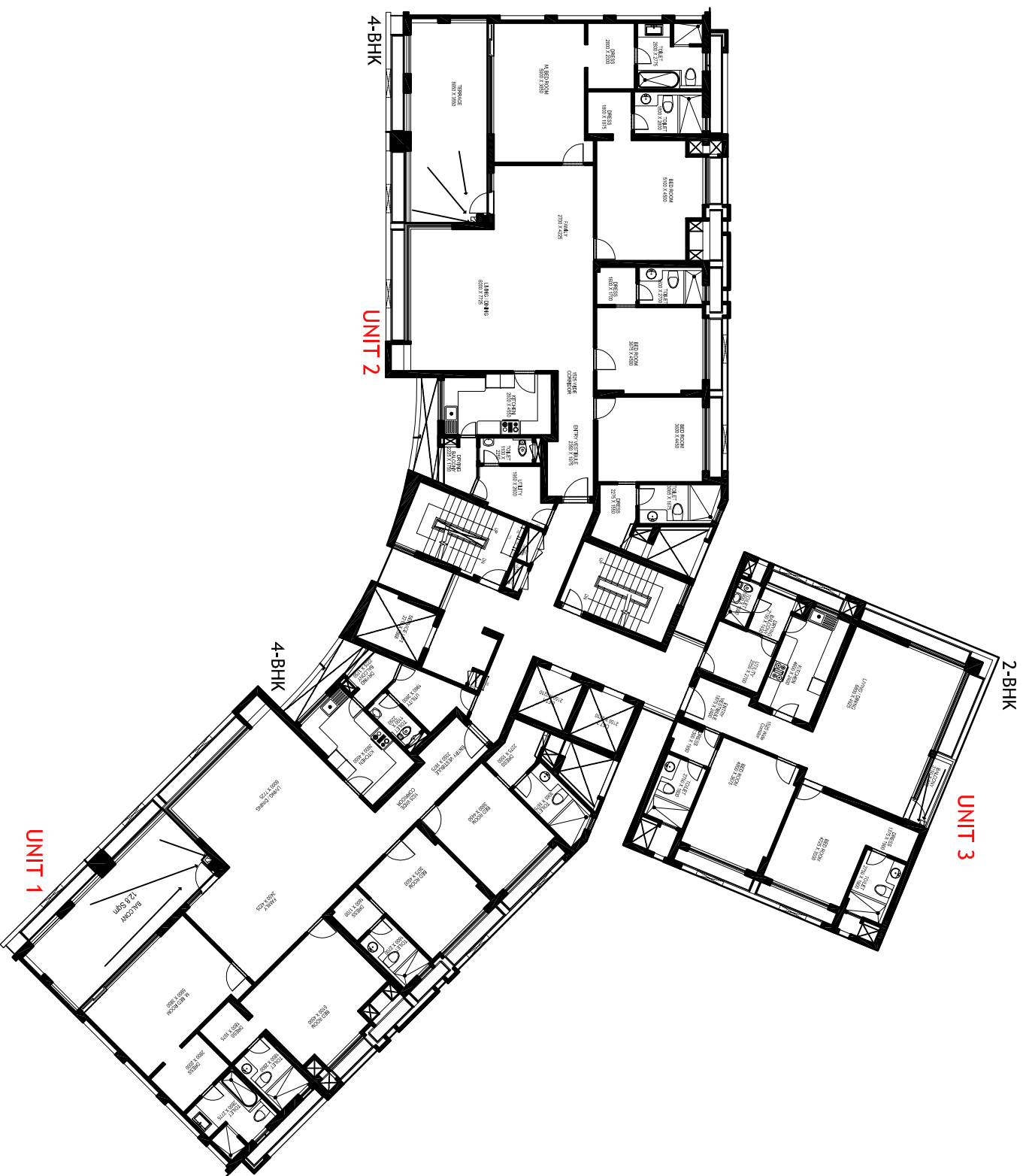
KALYPSO COURT-TOWER 7&8-5th, 13th & 21st FLOOR PLAN
