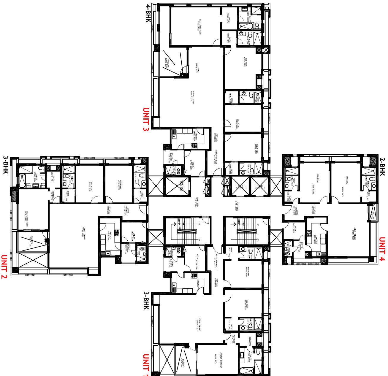
KALYPSO COURT-TOWER 10-3rd & 11th FLOOR PLAN
