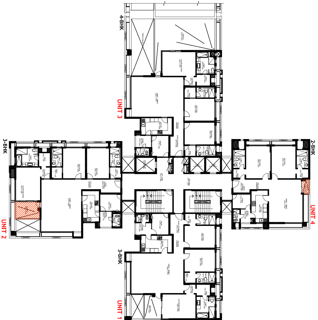
KALYPSO COURT-TOWER 10-6th & 14th FLOOR PLAN
