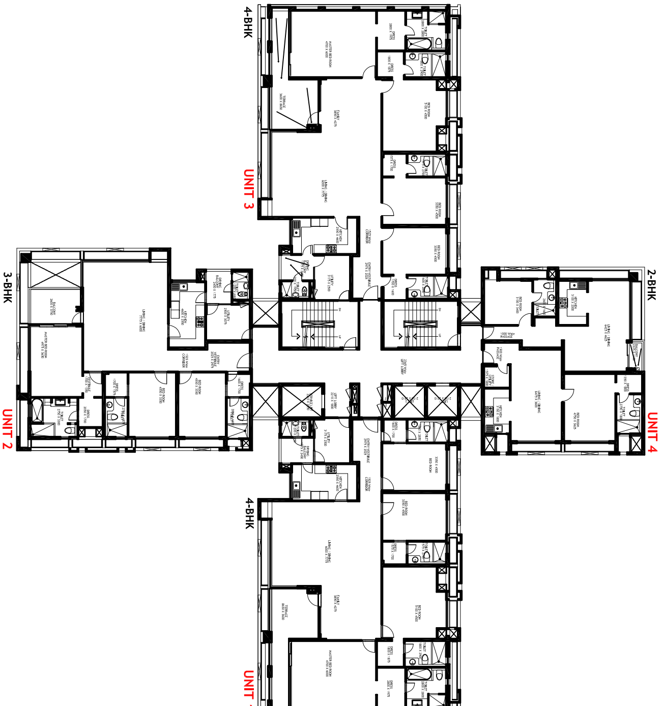
KALYPSO COURT-TOWER 9-3rd & 11th FLOOR PLAN
