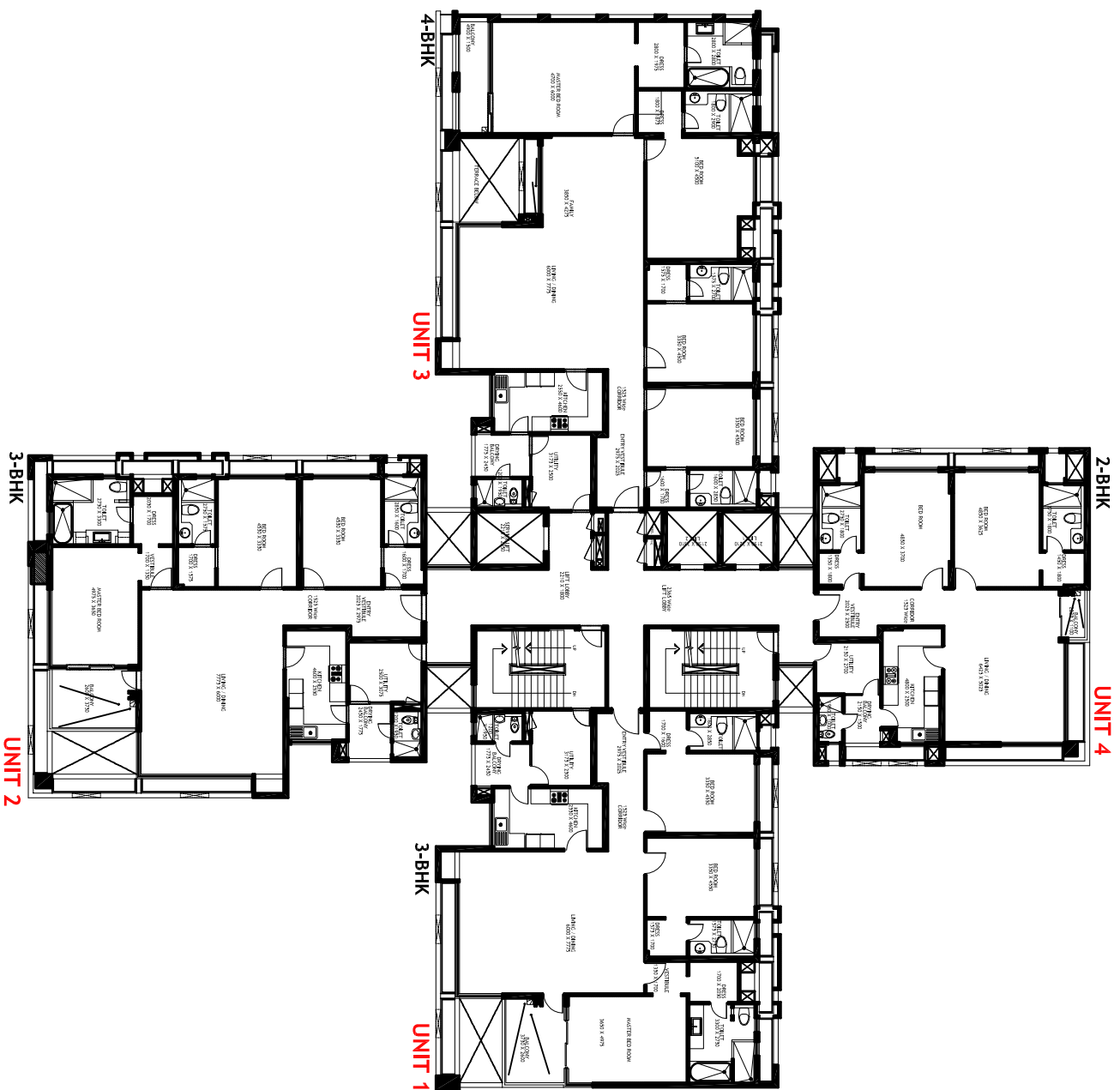
KALYPSO COURT-TOWER 10-4th & 12th FLOOR PLAN
