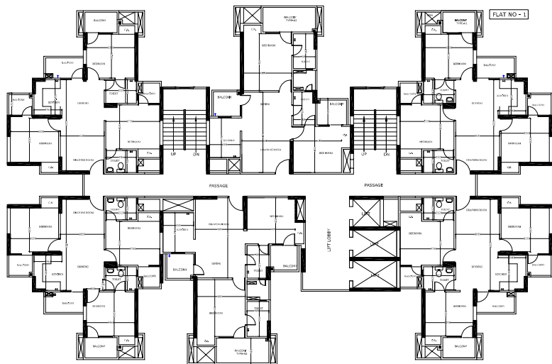
TOWER -J2 TYPICAL FLOOR PLAN
