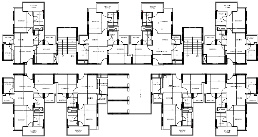
TOWER -12 TYPICAL FLOOR PLAN
