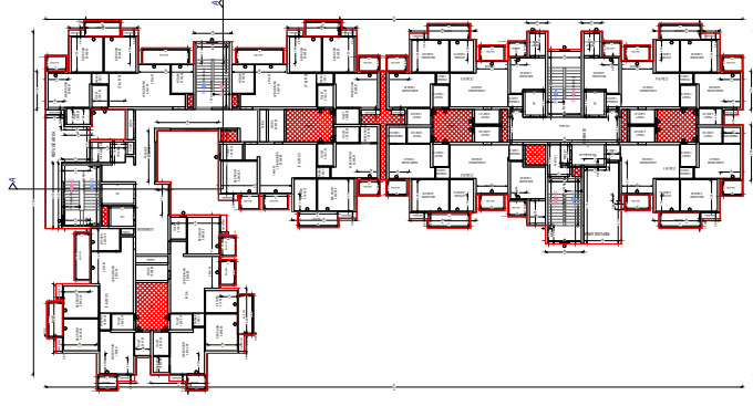
TYPICAL - 17 & 26 FLOOR PLAN (Proposed) (SCALE 1:100)
