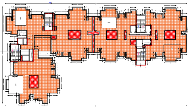
TERRACE FLOOR PLAN (SCALE 1:100)
