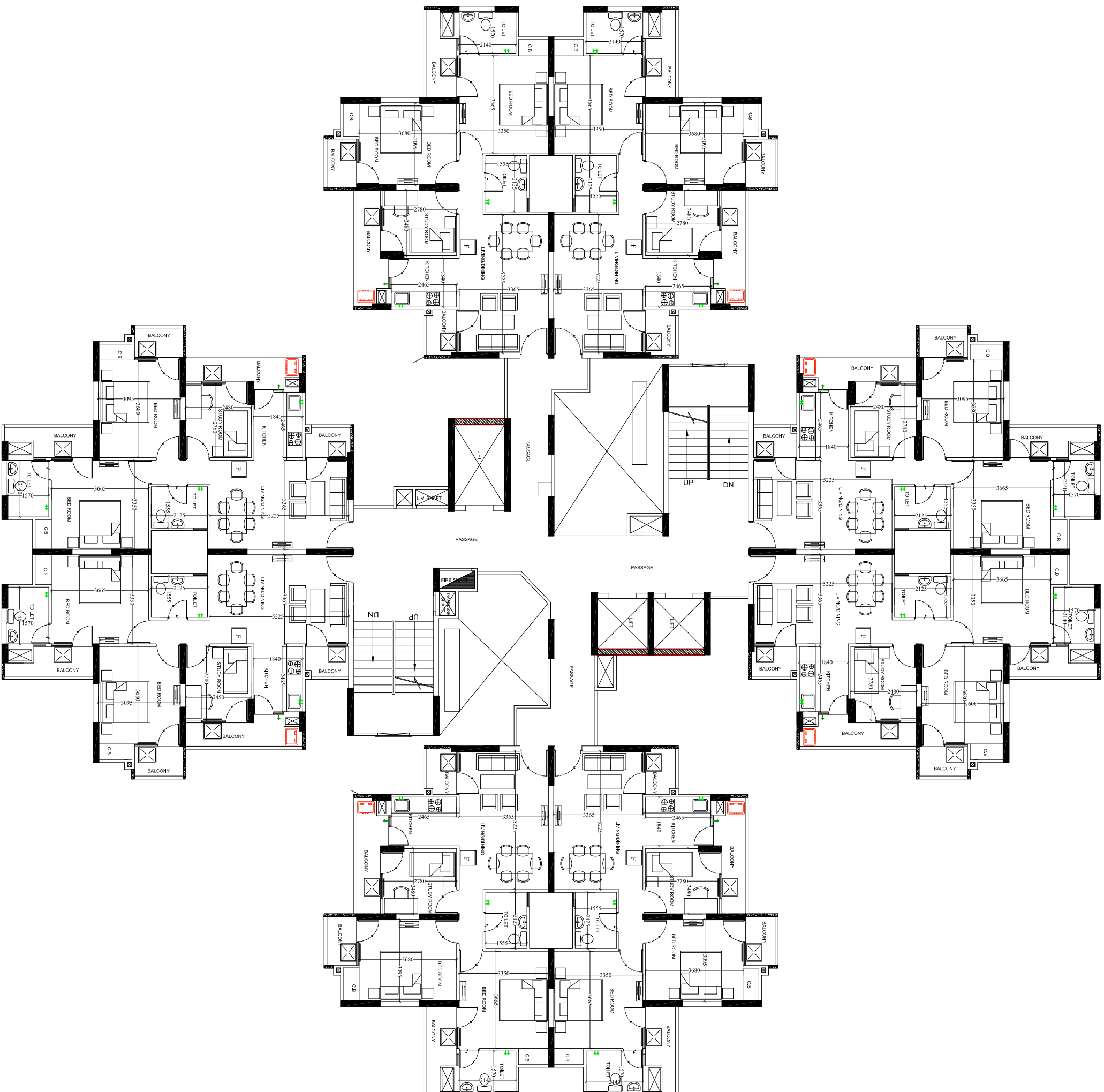
TOWER-C3,C4,C5 TYPICAL FLOOR
