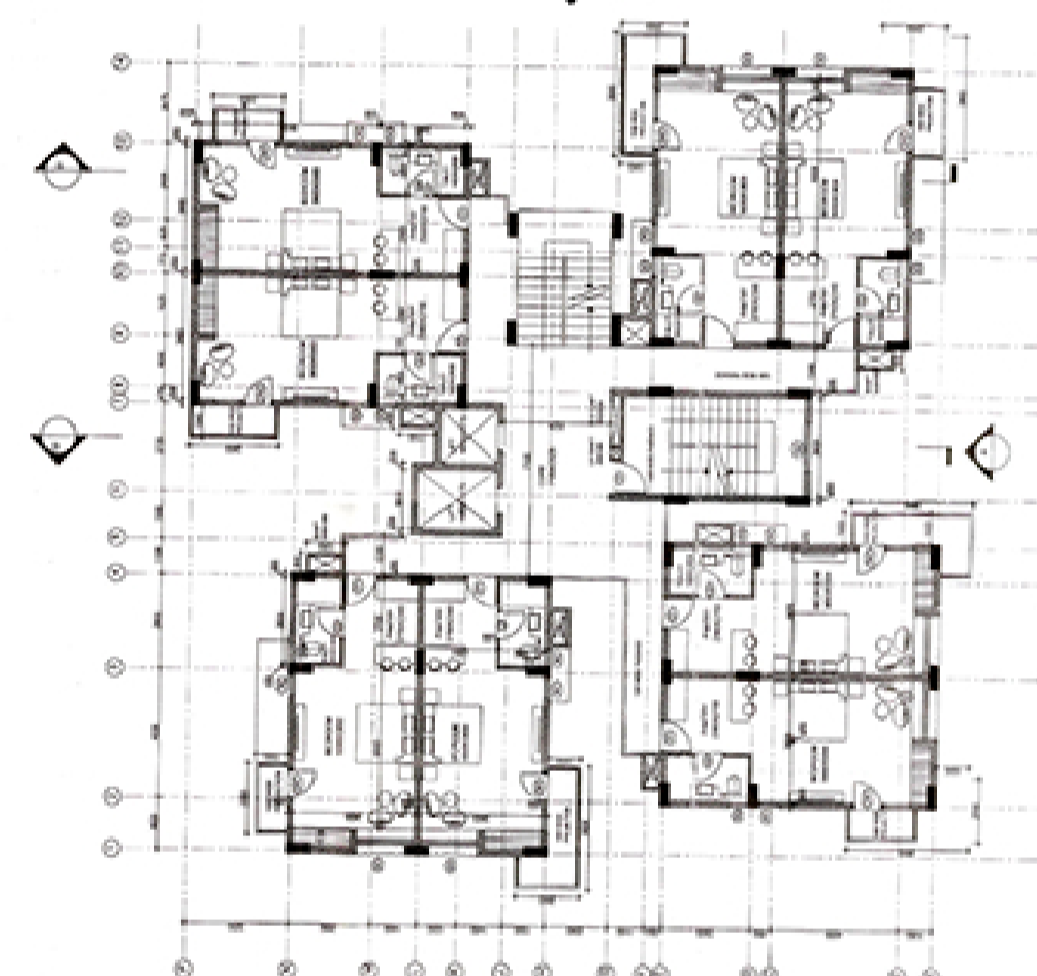
PLAN AT SECOND, FOURTH, SIXTH, EIGHTH, TENTH, TWELVETH & FORTENTH FLOORS
