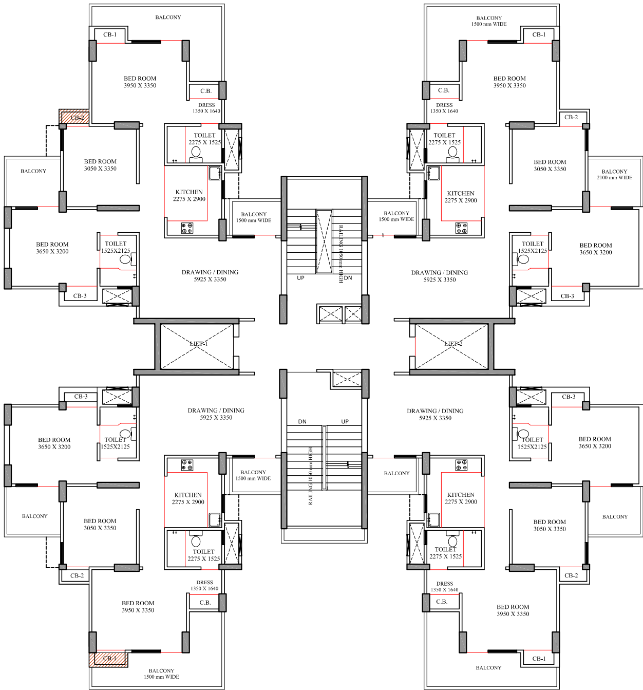
TOWER - D14 TYPICAL FLOOR PLAN
