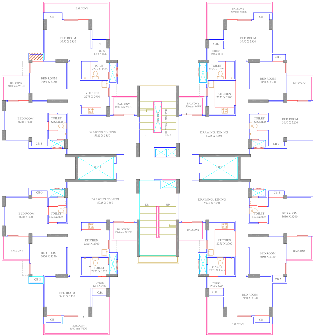
TOWER - D4 TYPICAL FLOOR PLAN
