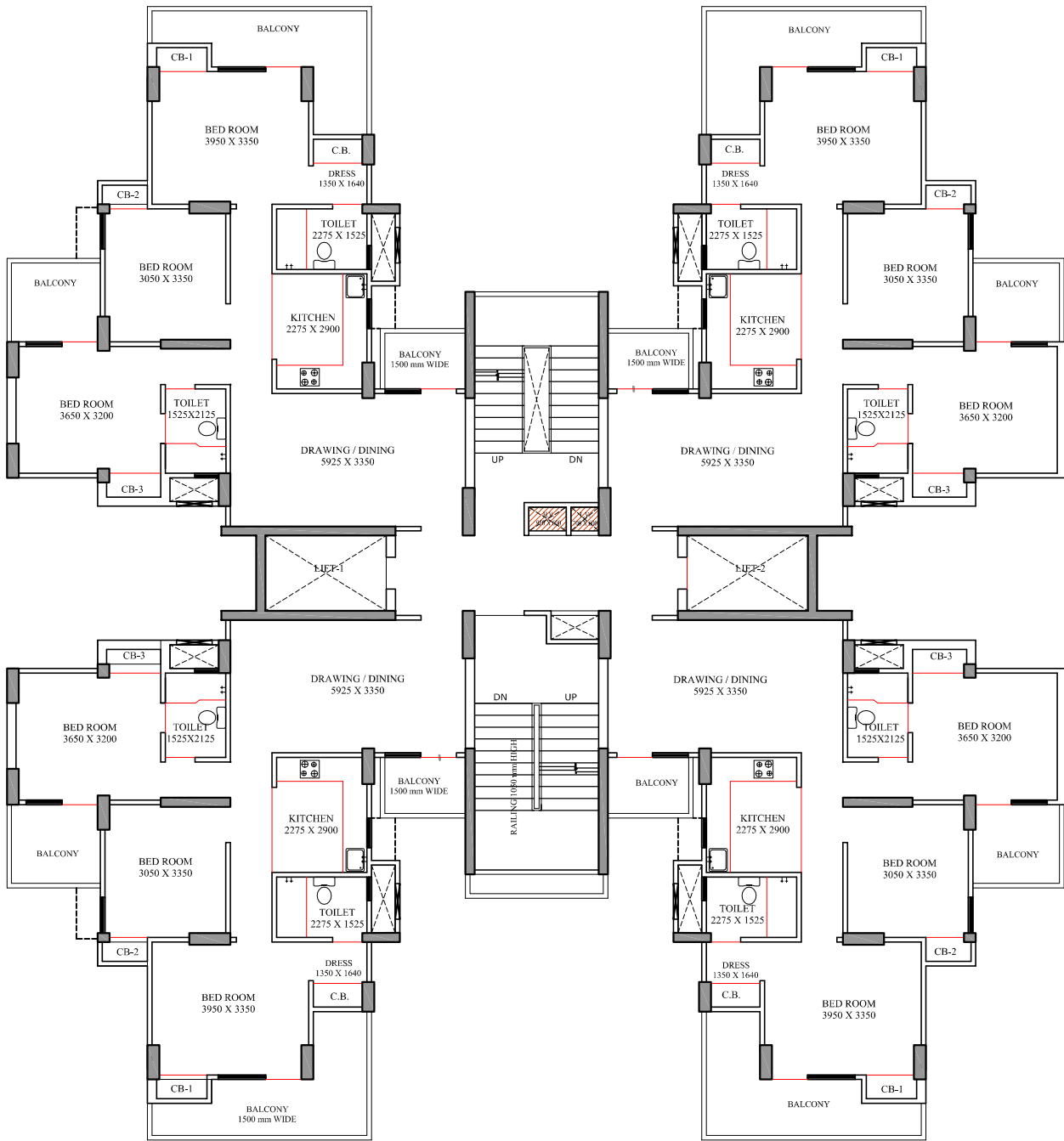
TOWER - D16 TYPICAL FLOOR PLAN
