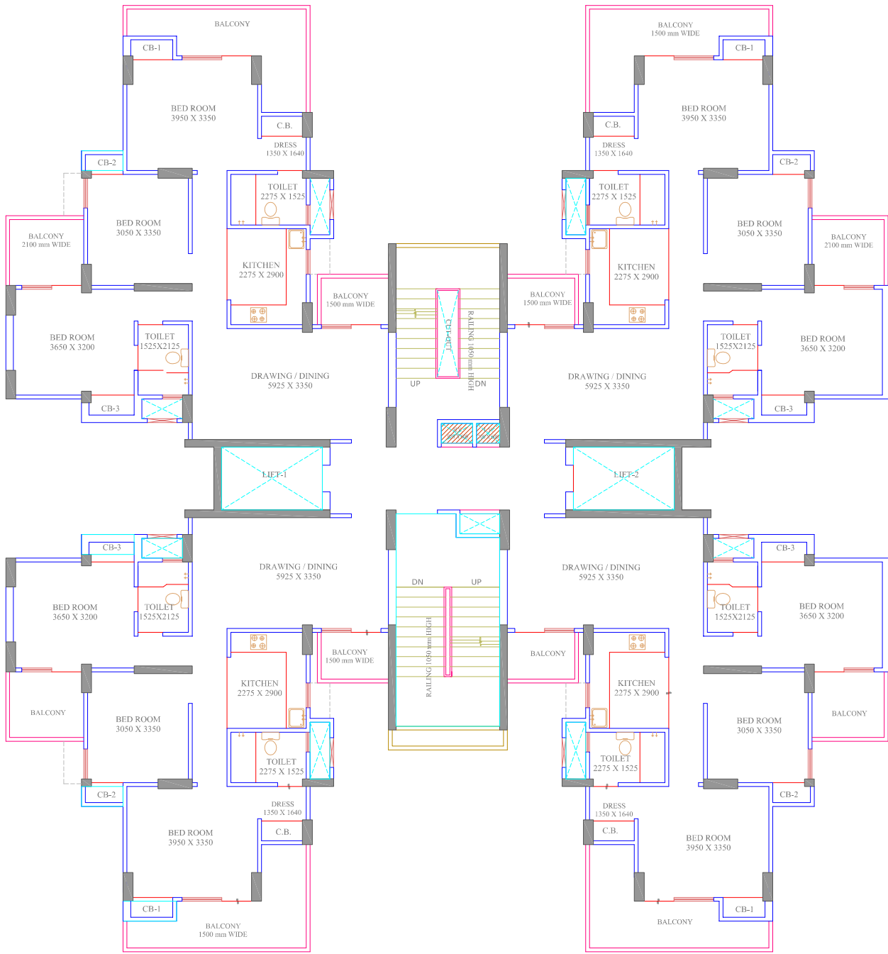
TOWER - D7 TYPICAL FLOOR PLAN
