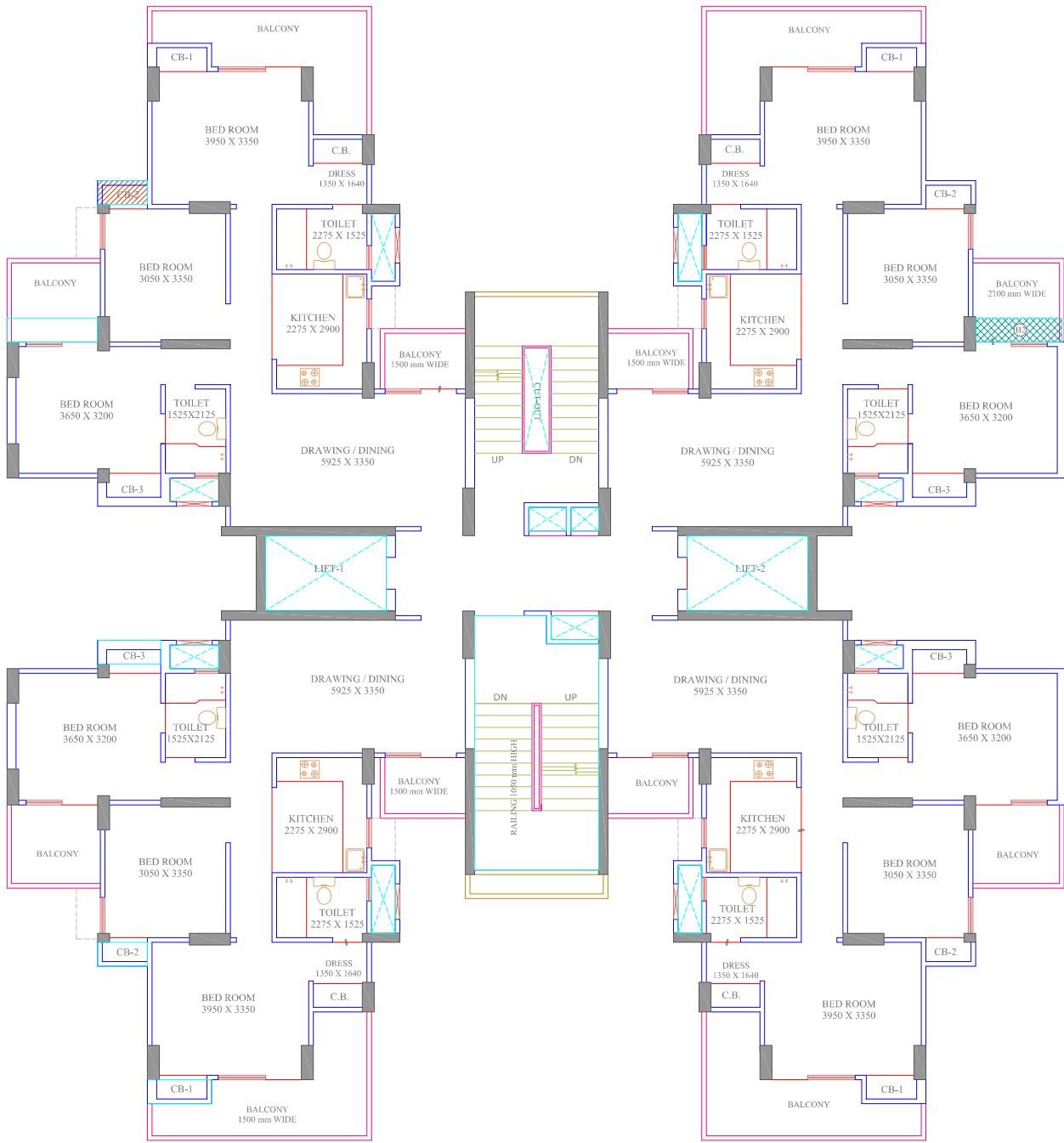
TOWER - D12A TYPICAL FLOOR PLAN
