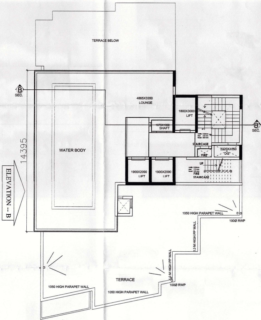
TOWER - CELESTE EUROPA PROPOSED 32nd FLOOR PLAN
