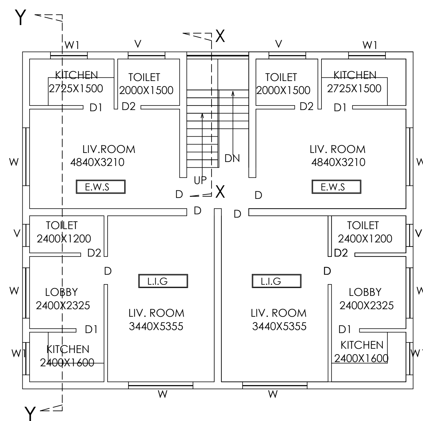
1st. AND 2nd.Floor Plan Scale = 1:100
