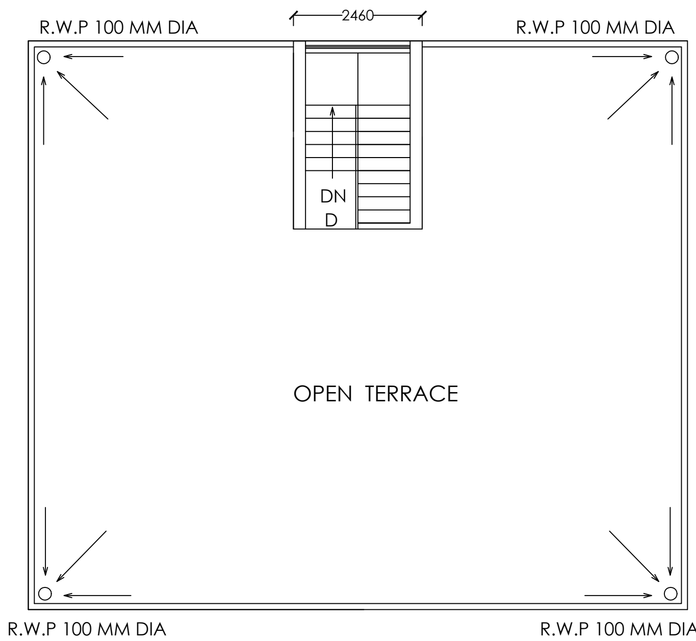
TERRACE Plan Scale = 1:100
