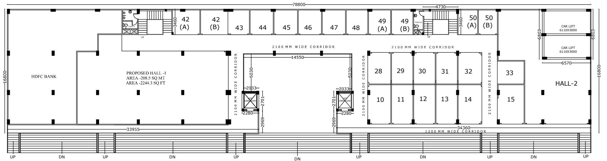
UPPER GROUND FLOOR PLAN
