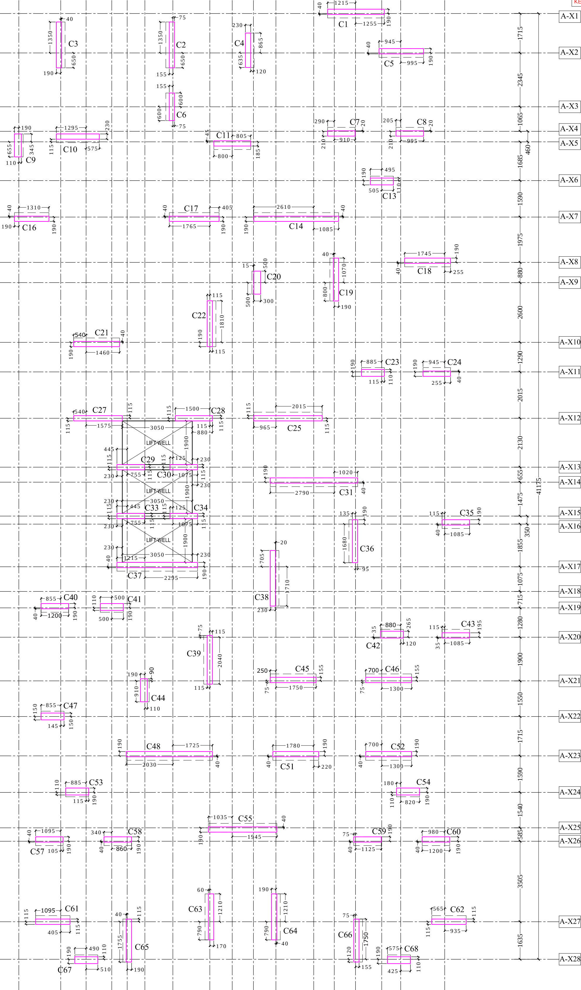
TOWER-A TYPICAL COLUMN GRID PLAN BUILDING HEIGHT IS [2 BASEMENT +G+ 22 STOREY]
