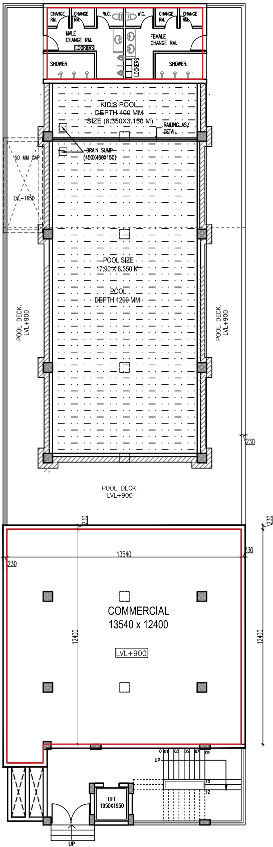
GROUND FLOOR PLAN POOL DECK @ +900 LVL.
