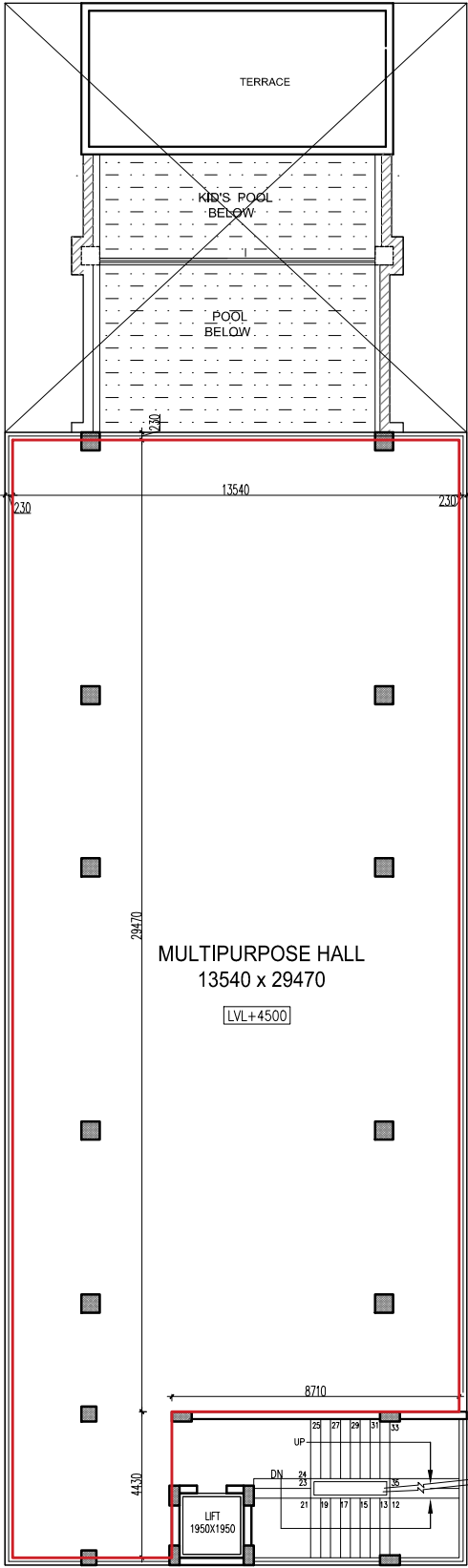
FIRST FLOOR PLAN (@ 4500 LVL.)
